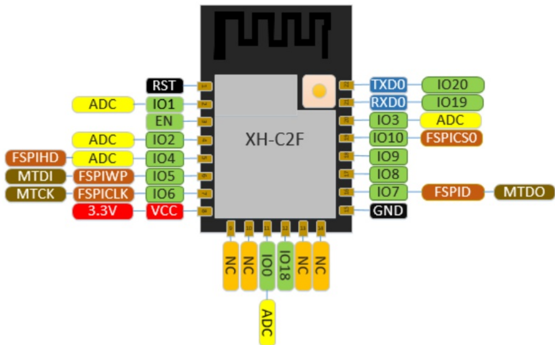
Fig. 2.1 XH-C2F Pin Definition
