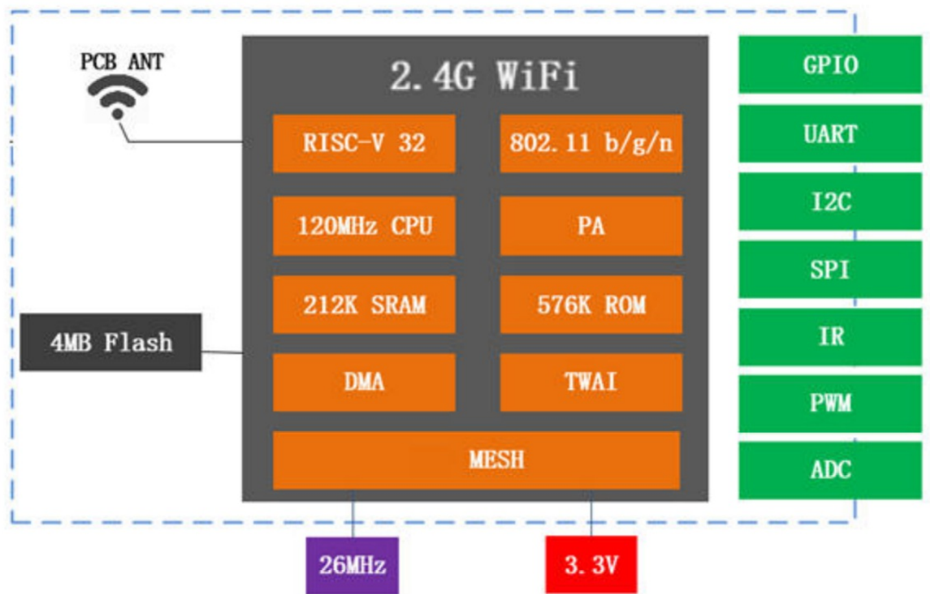
Fig. 1.1 XH-C2F Module Structure
