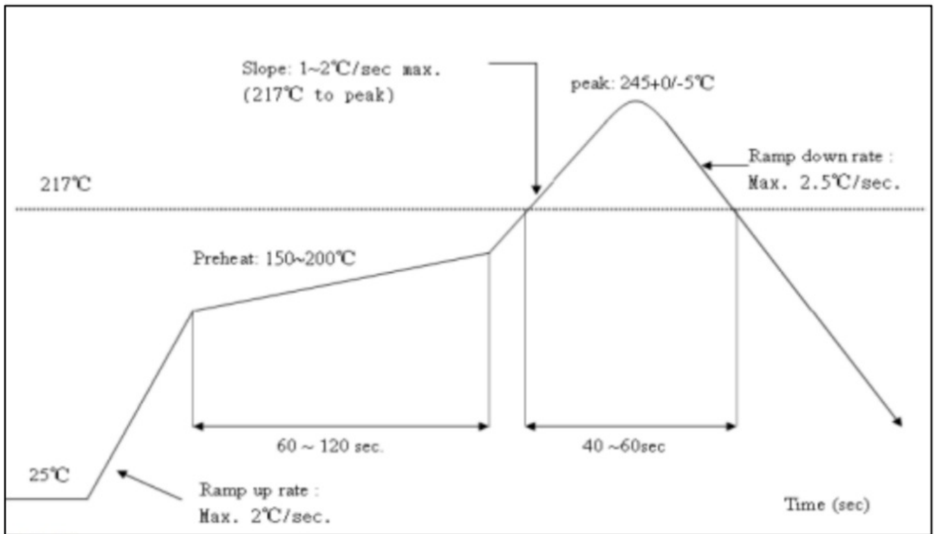
图 7.1 Temperature Curve when sold
