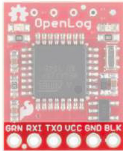
Serial Connection Header.
