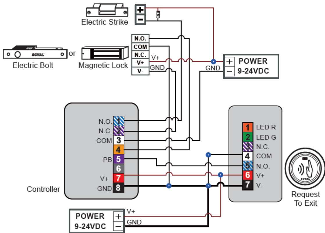
The Wiring Diagram of LED R/G Door Status Indication
