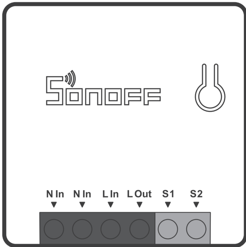
Wi-Fi Smart Switch with Diy Mode
