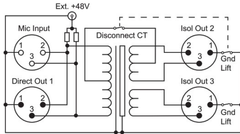
Fig 1-2: CM-MS3 Block Diagram
