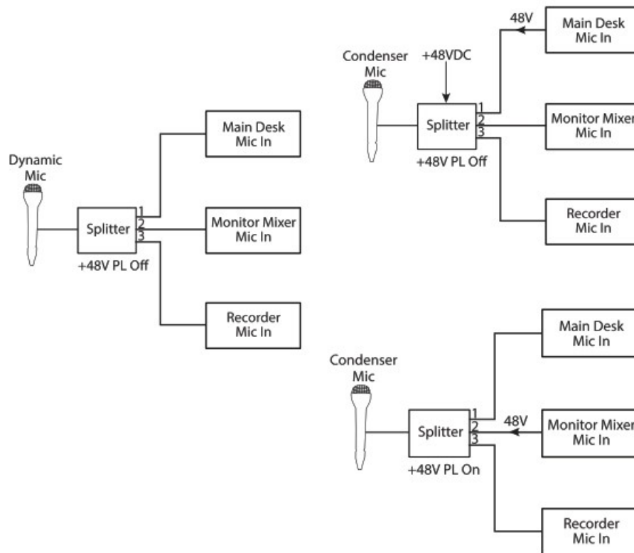
Fig 1-3: CM-MS3 Examples of Usage
