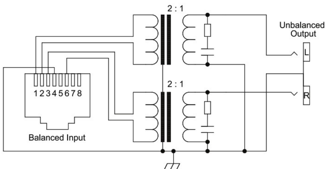
Fig 1-3: CM-LUR1 Block Diagram
