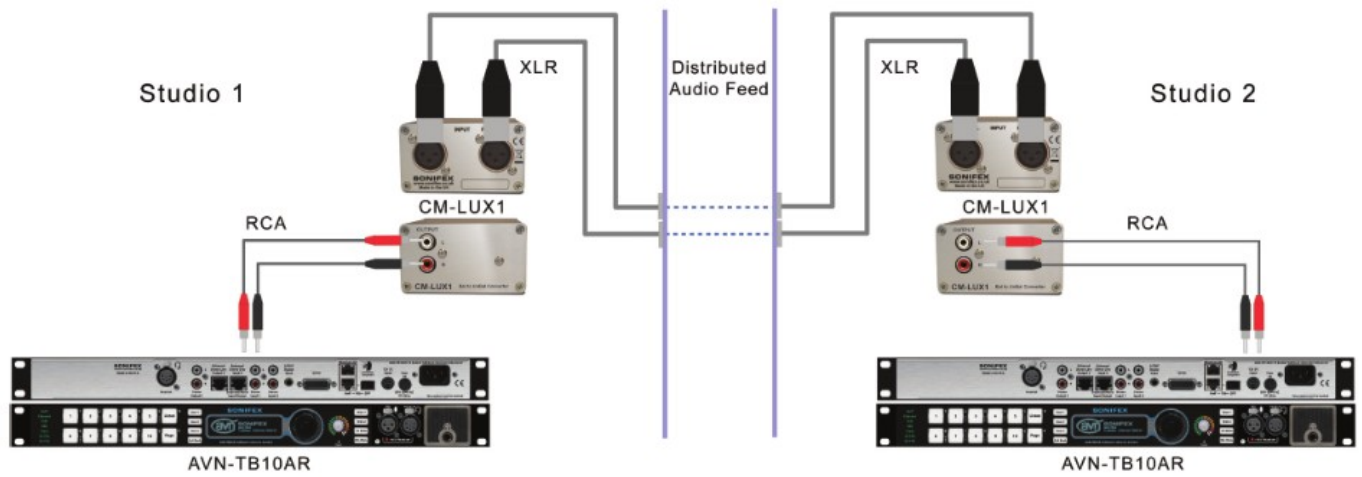
Fig 1-5: CM-LUX1 Application Diagram
