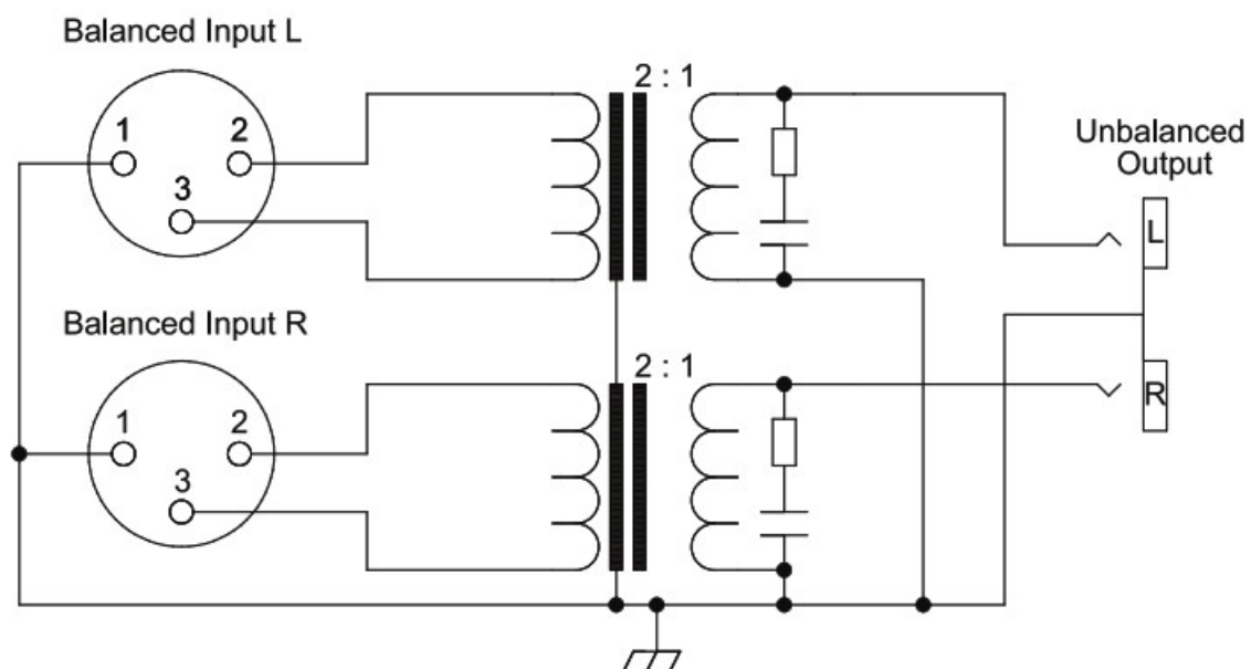
Fig 1-4: CM-LUX1 Block Diagram
