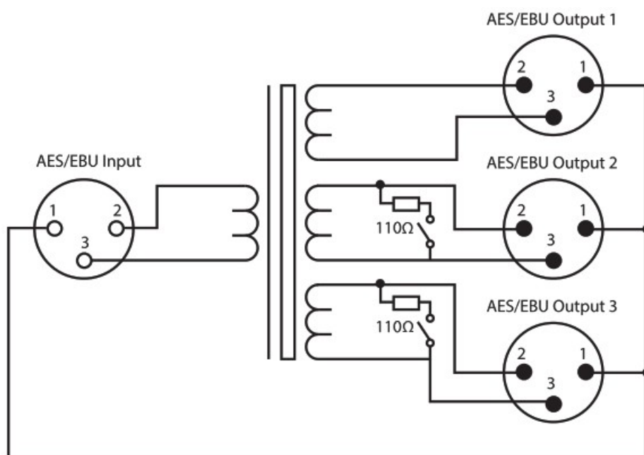
Fig 1-2: CM-AESX3 Block Diagram
