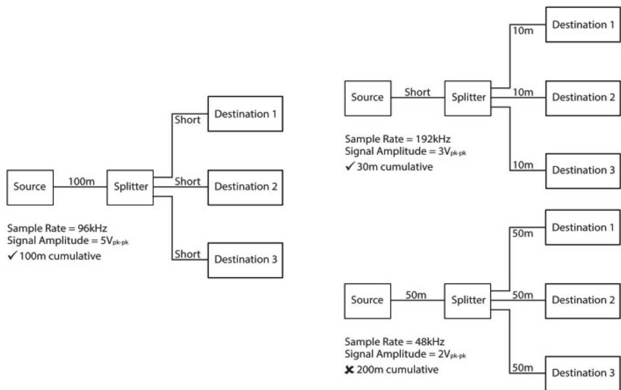
Fig 1-3: CM-AESX3 Examples of use of Cumulative Cabling
