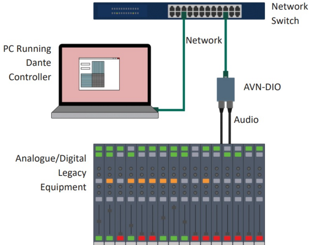
Fig 2: Typical AVN-DIO setup
