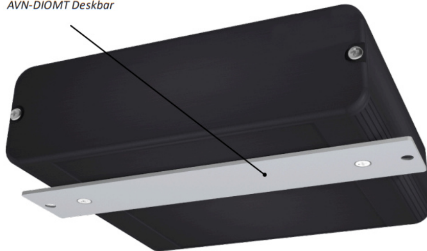
Fig 1-6: Iso View Shown with AVN-DIOMT Deskbar Attached
