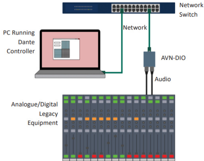
Fig 3: Typical AVN-DIO setup
