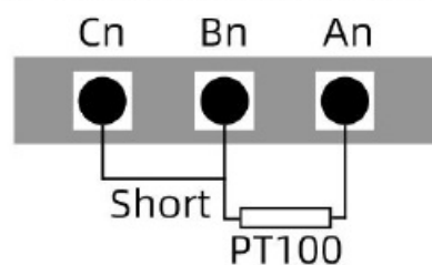
Two-wire connection
