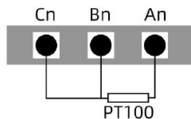
Three-wire connection
