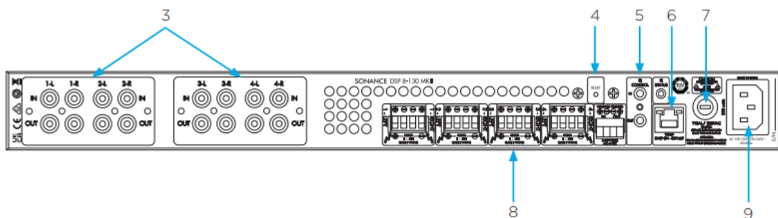
Figure 4: DSP 8-130 MKIII Multi-Channel Power Amplifier Rear Panel
