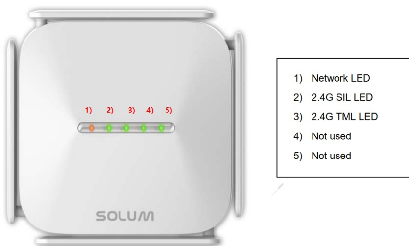
Figure 4.4. Gateway LEDs
