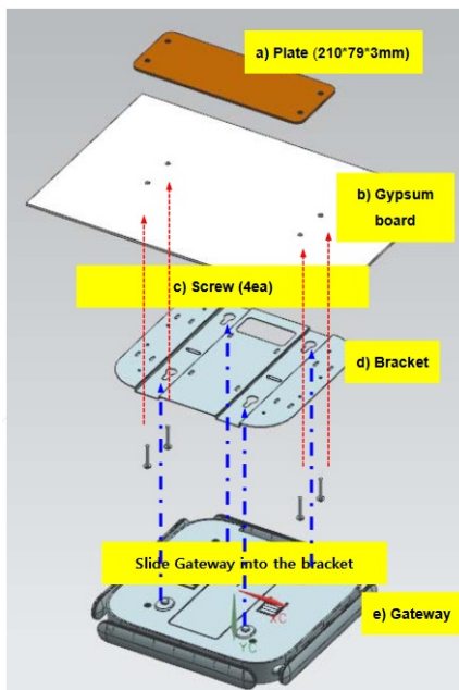
Figure 5.1. Gateway Installation
