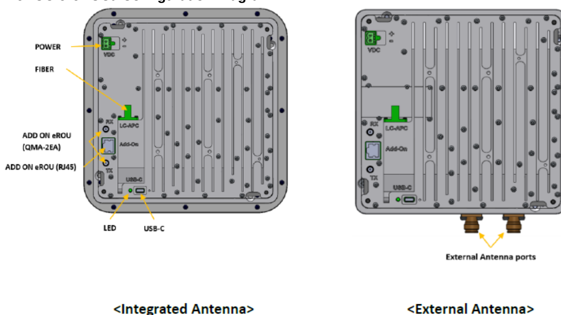
Figure 2. eROU outer Look
