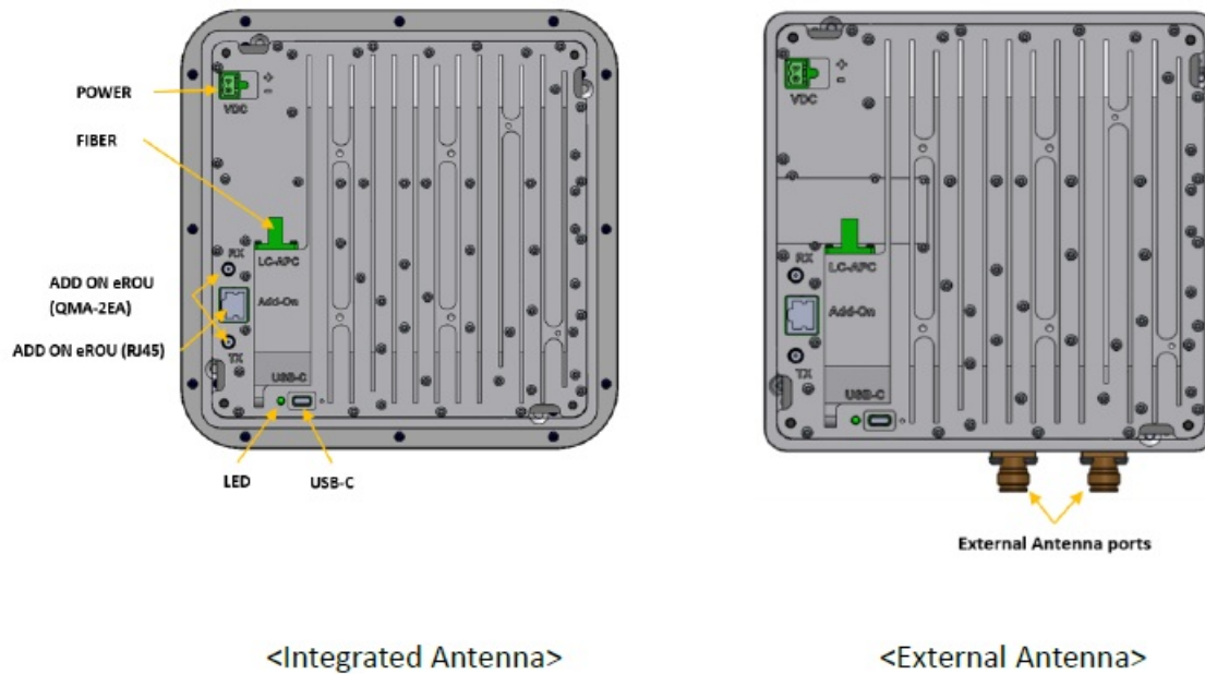
Figure 4. The name of each port on eROU
