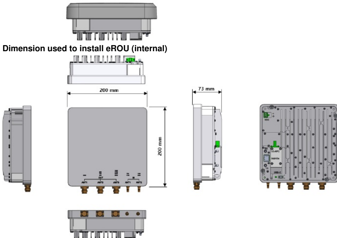
Figure 3. Dimension used to install eROU (external)
