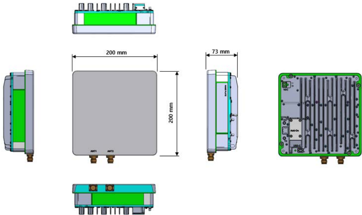
Figure 4. Dimension used to install eROUa (external)
