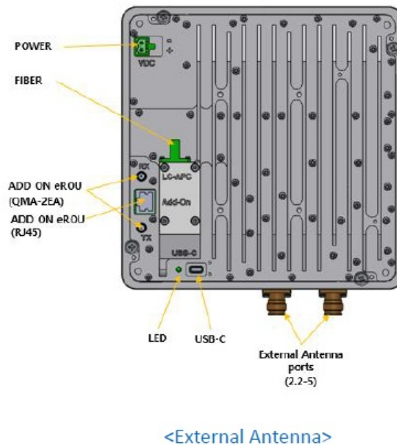
Figure 5. The name of each port on eROUa
