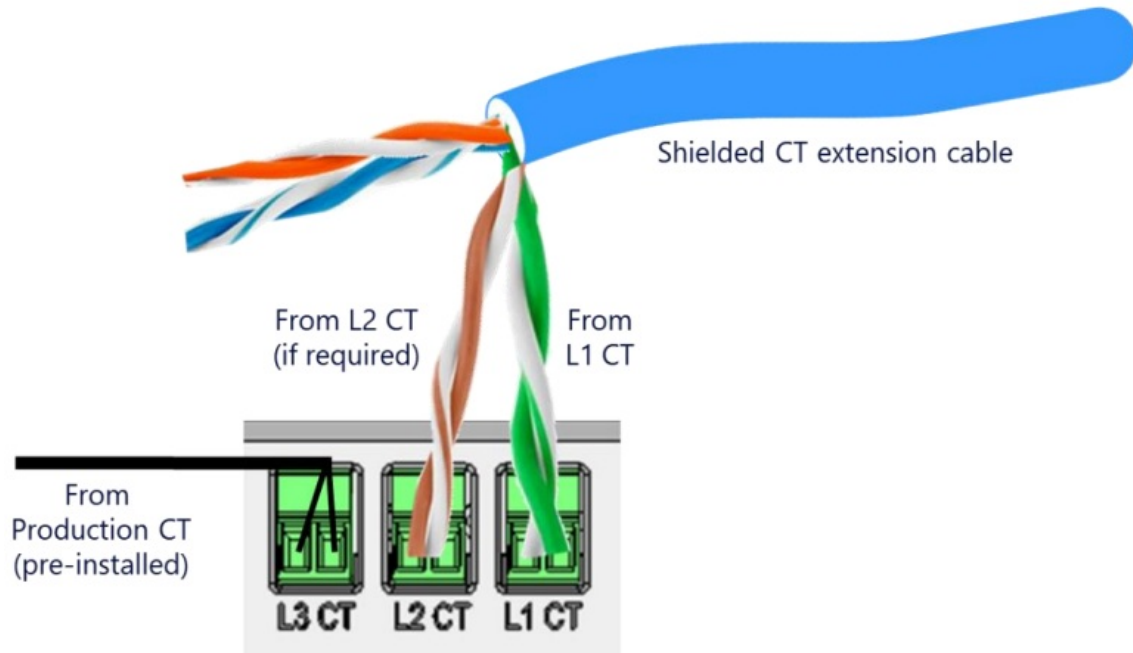
Figure 5: Connecting the CT Wires to the Meter
