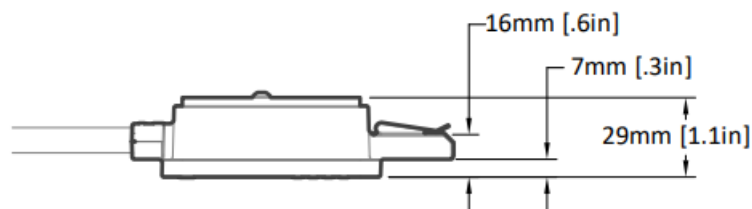
Figure (3.4) Side view of the O900-80V with the measurements of its sides, not including the cables and connectors.
