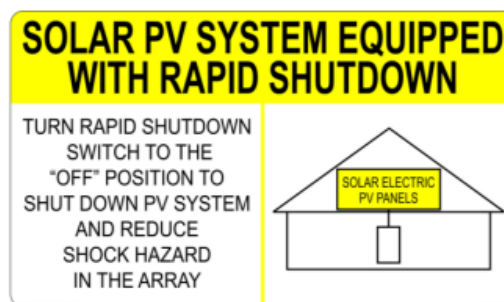
Figure (2.2) Rapid Shutdown System Label, NEC 690.12 (C)
