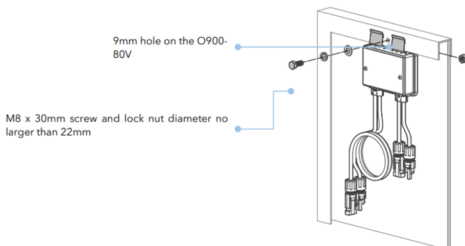
Figure (3.5) Mounting the O900-80V on a frameless solar panel
