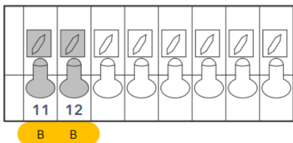
Figure (2.1) Terminal board for sensors on the Sol-Ark 12K-2P-N
