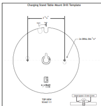
*Table Mounting Template
