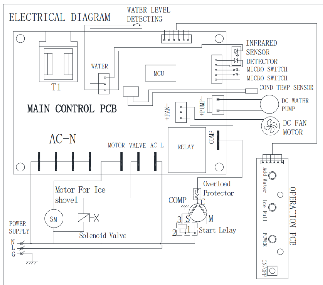
ELECTRICAL DIAGRAM
