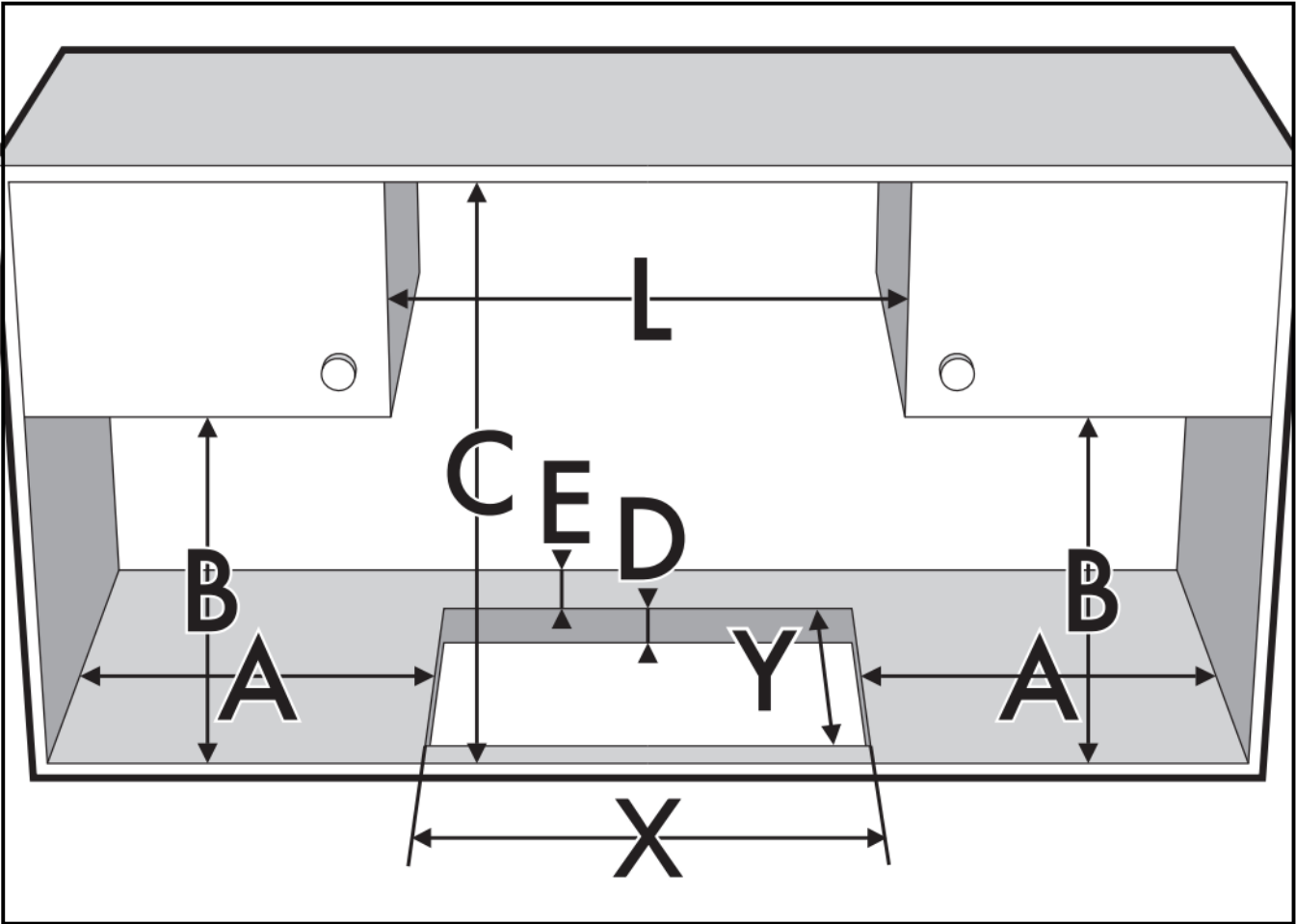
Built-in cabinet dimensions (mm)
