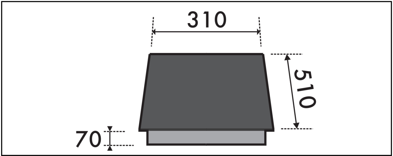
Built-in cabinet dimensions (mm)
