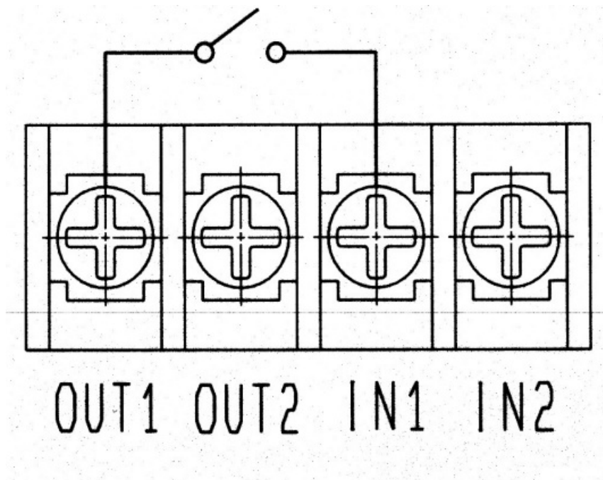
Fig. 21. Wiring for temporary stop
