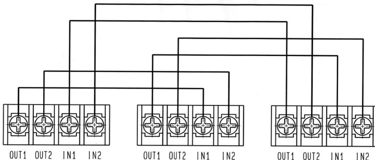
Fig. 12 Cascade connection
