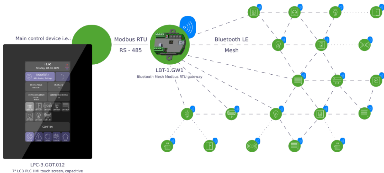
Figure 3: Bluetooth Mesh system topology
