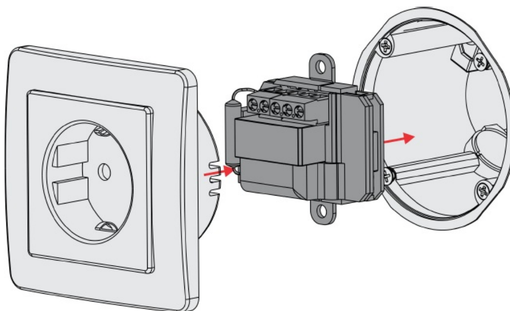
Figure 7: Mounting in flush mounting box
