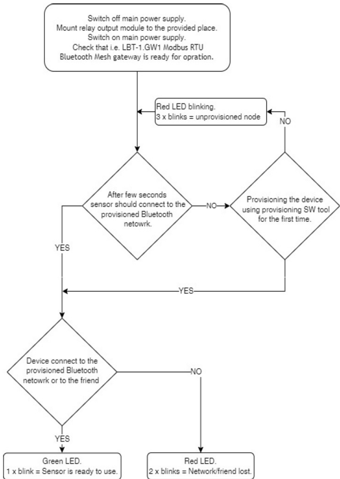
Figure 8: Installation flowchart
