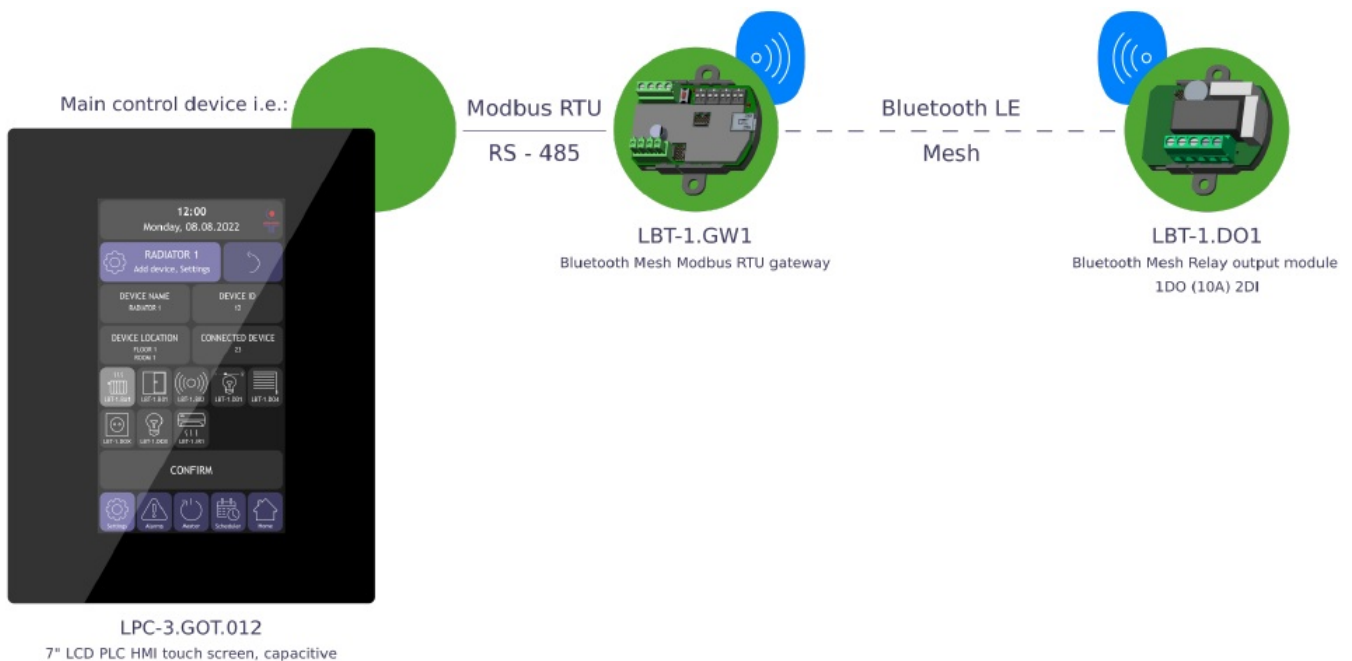
Figure 2: LBT-1.DO1 device connection
