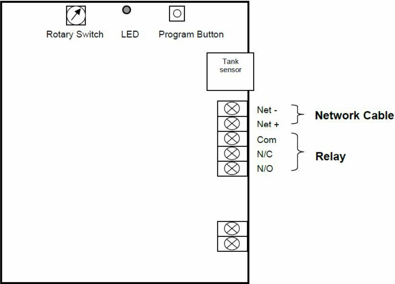
Wiring Diagram for Model HB-200
