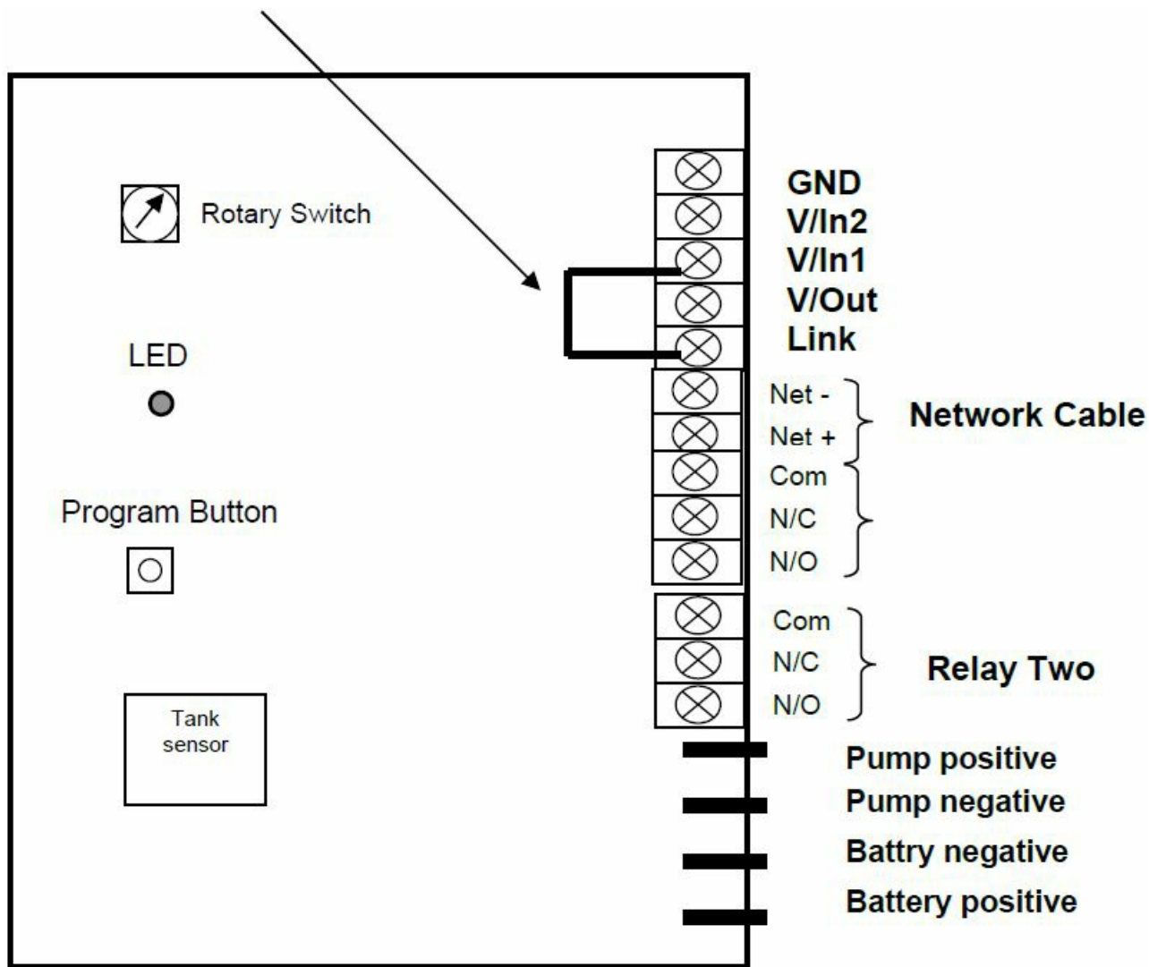
Wiring Diagram for Model HB-200/P
