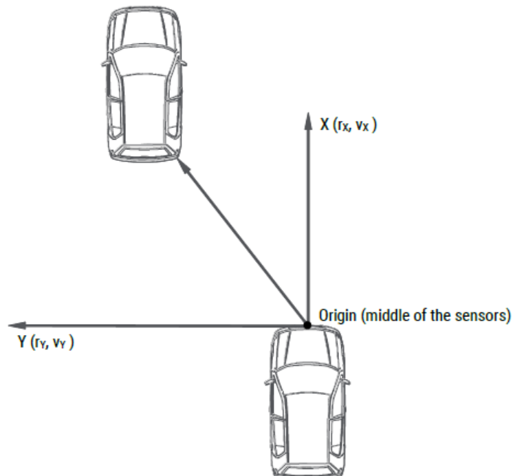
Figure 7: Sensor coordinate system
