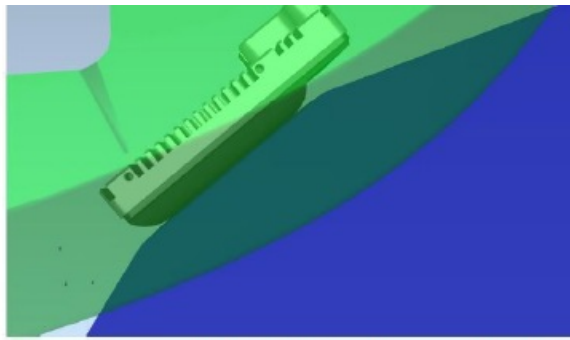
Figure 11: Example mounting position behind a bumper showing azimuth clearance (connector pointing to the center of the vehicle)
