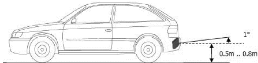
Figure 6: Typical mounting position - elevation angle
