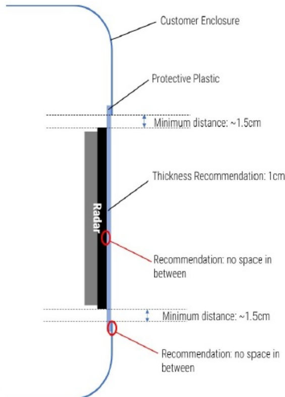
Figure 10: Material recommendation and placement overview
