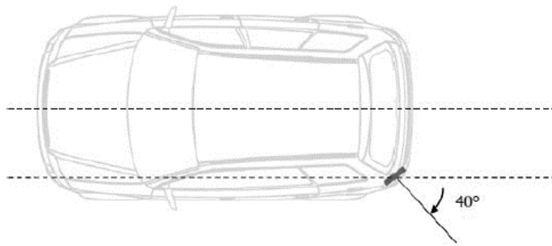
Figure 5: Typical mounting position - azimuth angle
