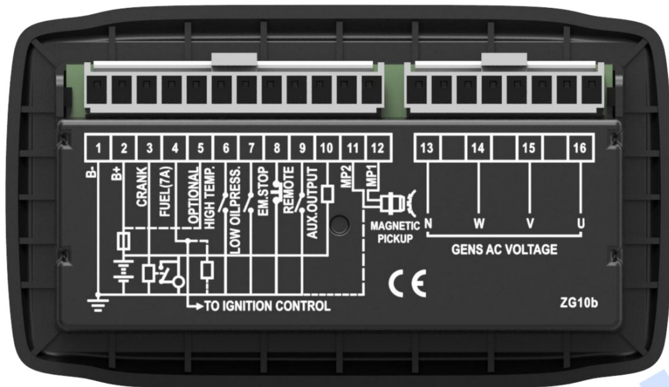
Fig.2 Rear Panel
