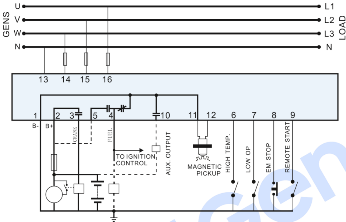
Fig.4 Typical Application
