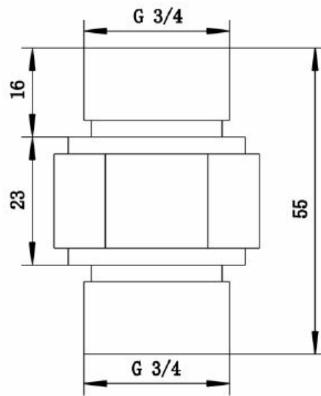
Fig. 9 Pair Screw Size
