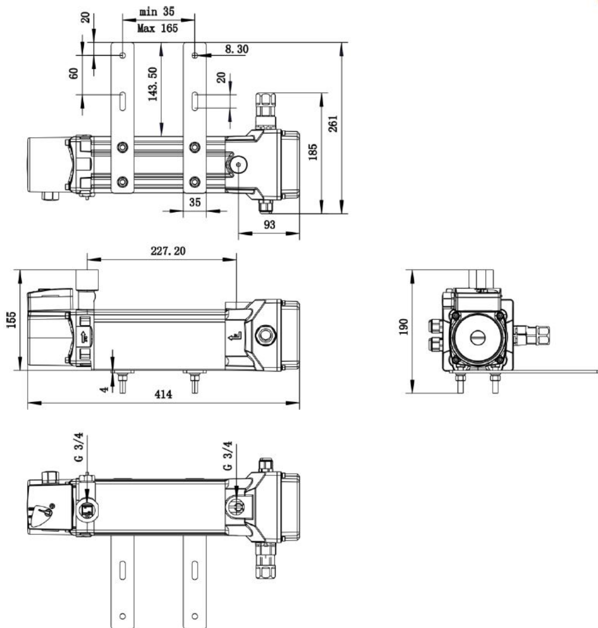
Fig. 7 – Overall Dimensions
