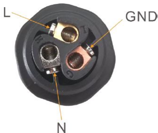
Fig. 5 Wire Connection
