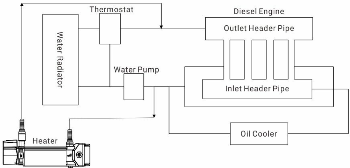
Fig. 1 – Installation Logic Diagram
