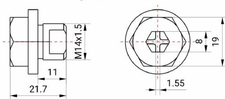
Fig. 6 Vent Valve Size
