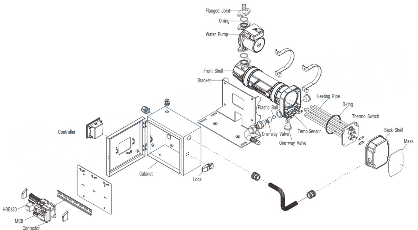
Fig. 4 – Assembly Structure
