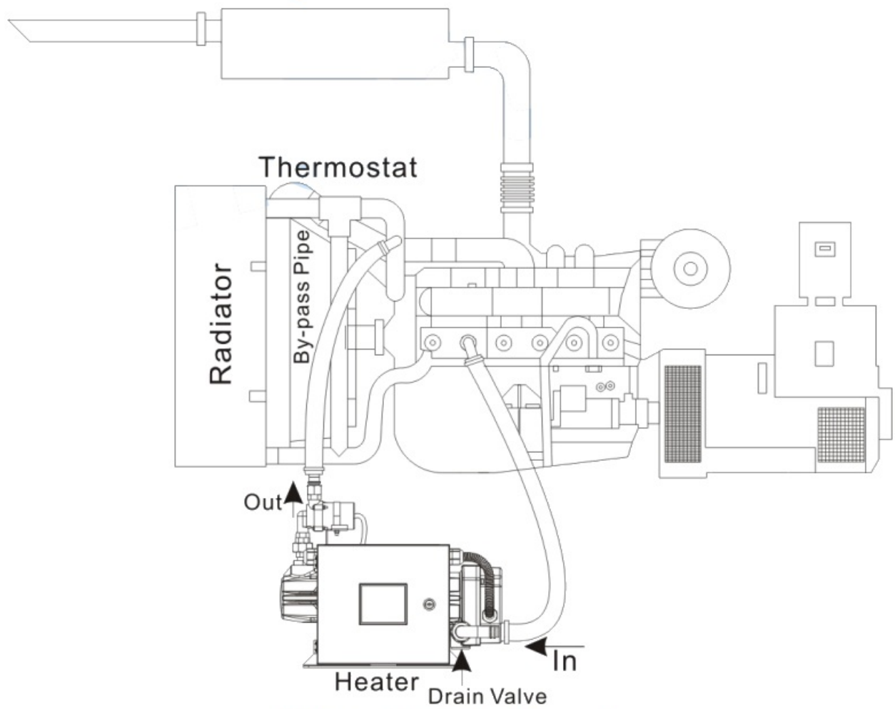
Fig.2 - Installation Side Schematic
