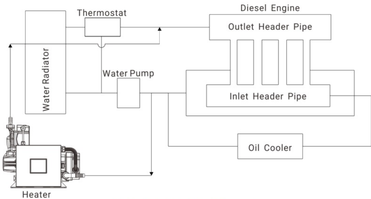
Fig.1 - Installation Plane Schematic
