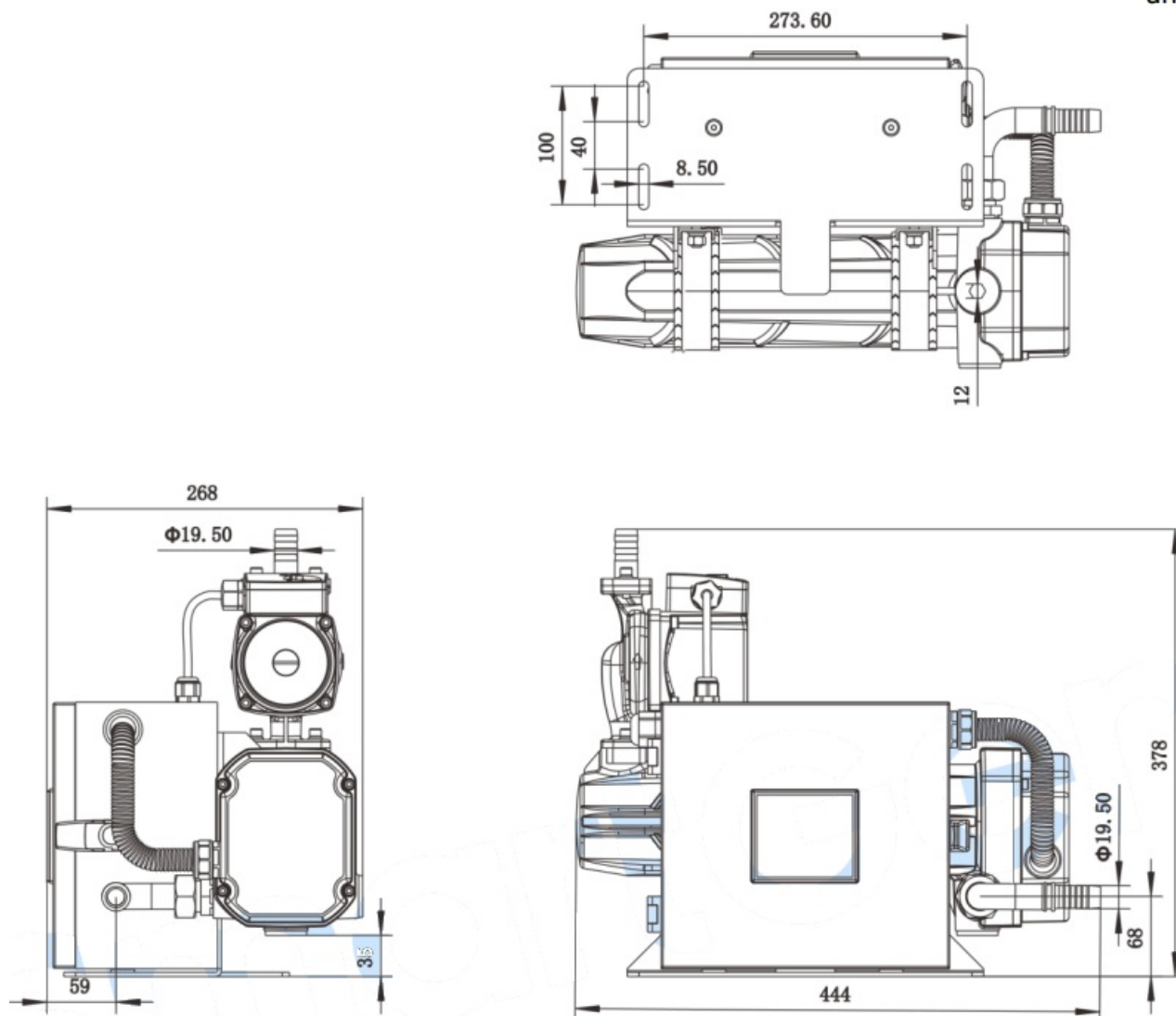
Fig.10 – Overall Dimensions
