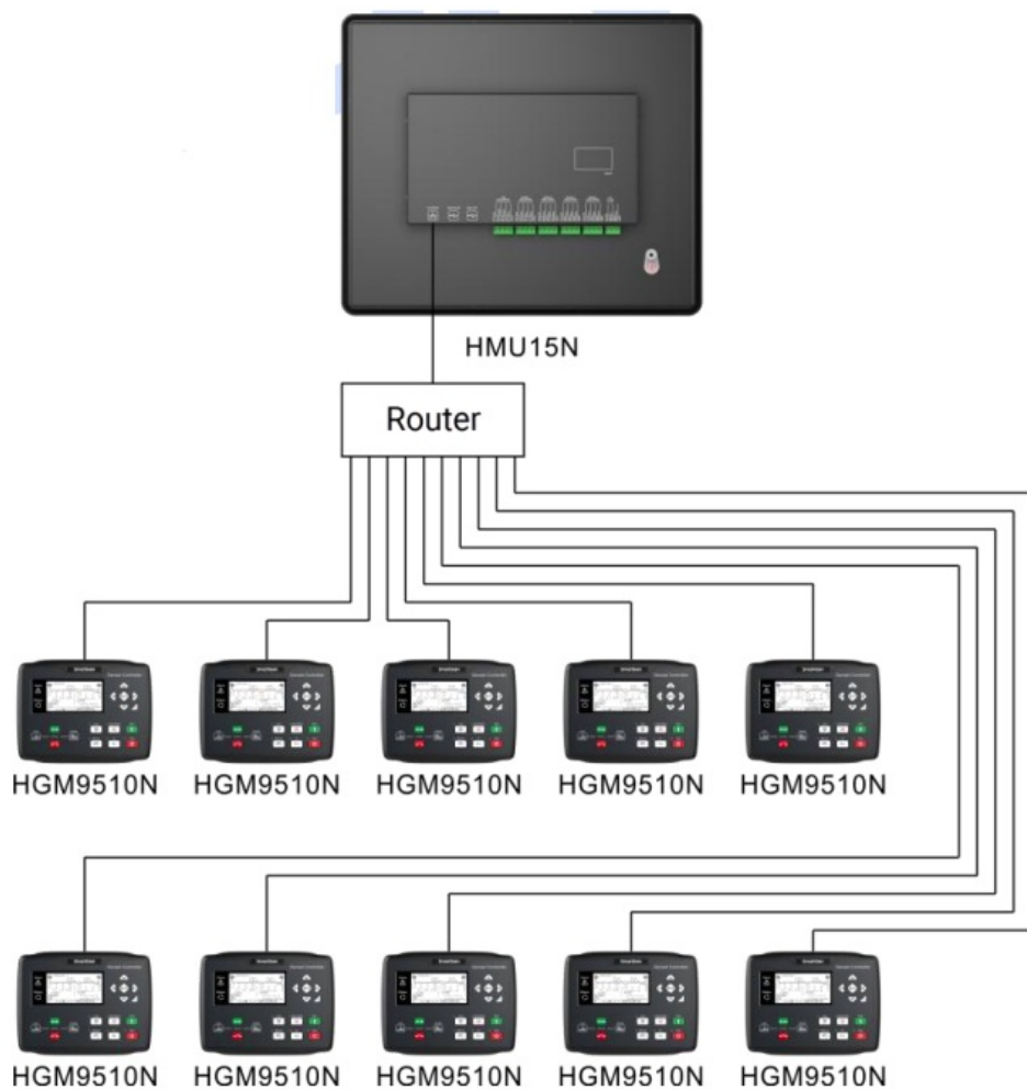
Fig.15 – Typical Application Diagram 2
