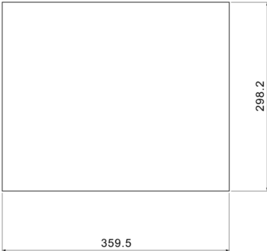
Fig.16 – Case Dimensions and Panel Cutout
