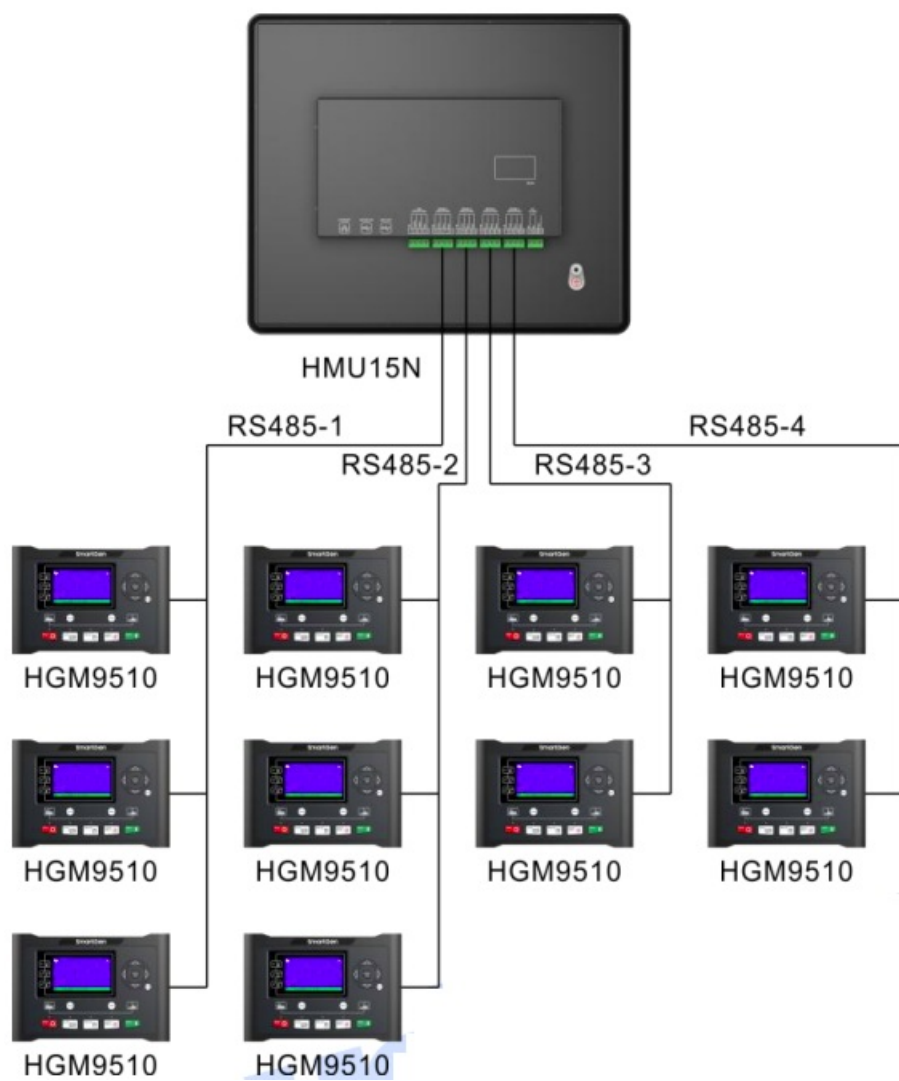
Fig.14 – Typical Application Diagram 1
