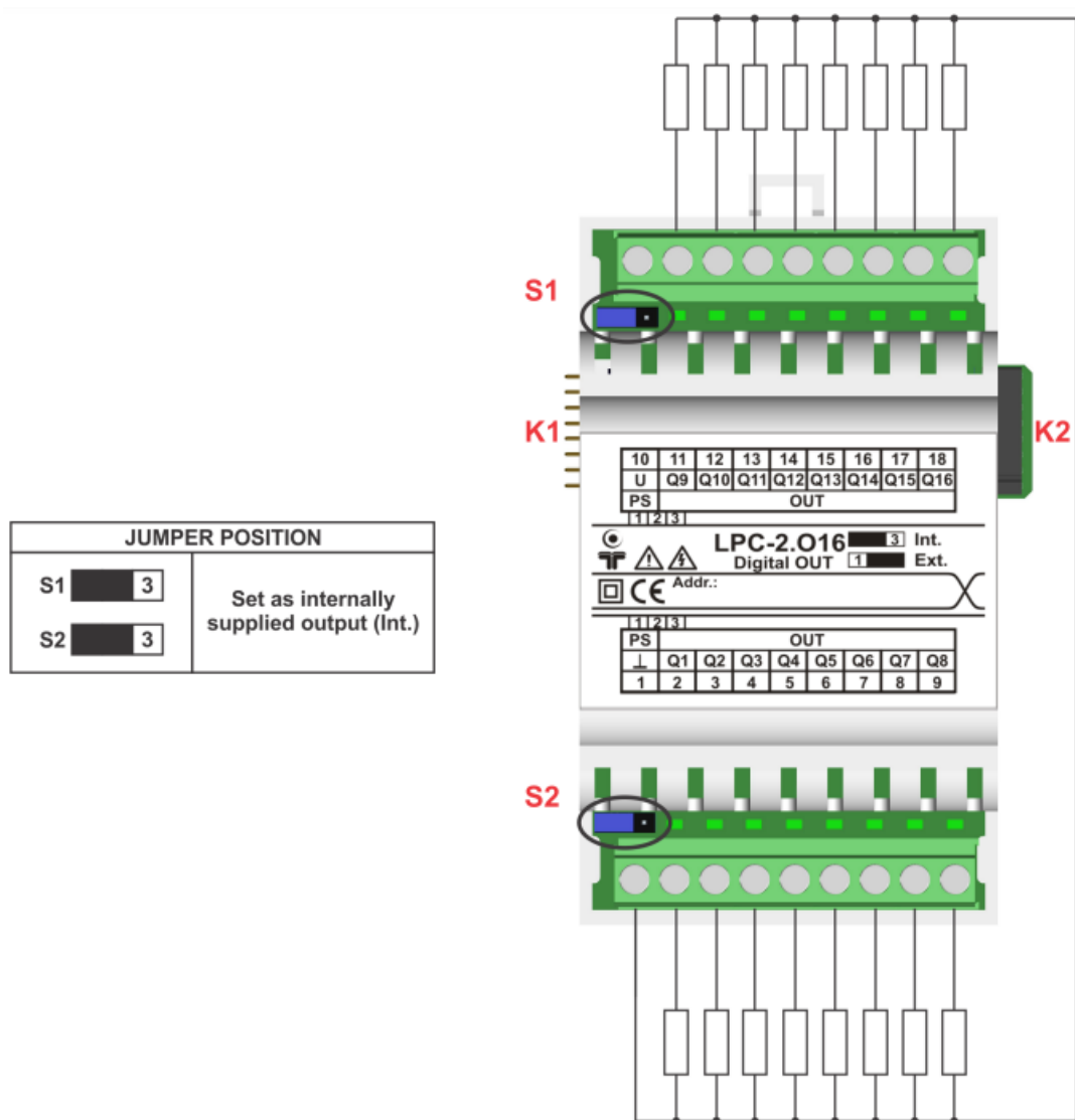
Figure 3: Connection scheme for externally supplied
