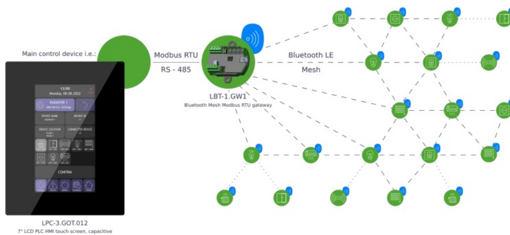
Figure 3: Bluetooth Mesh system topology
