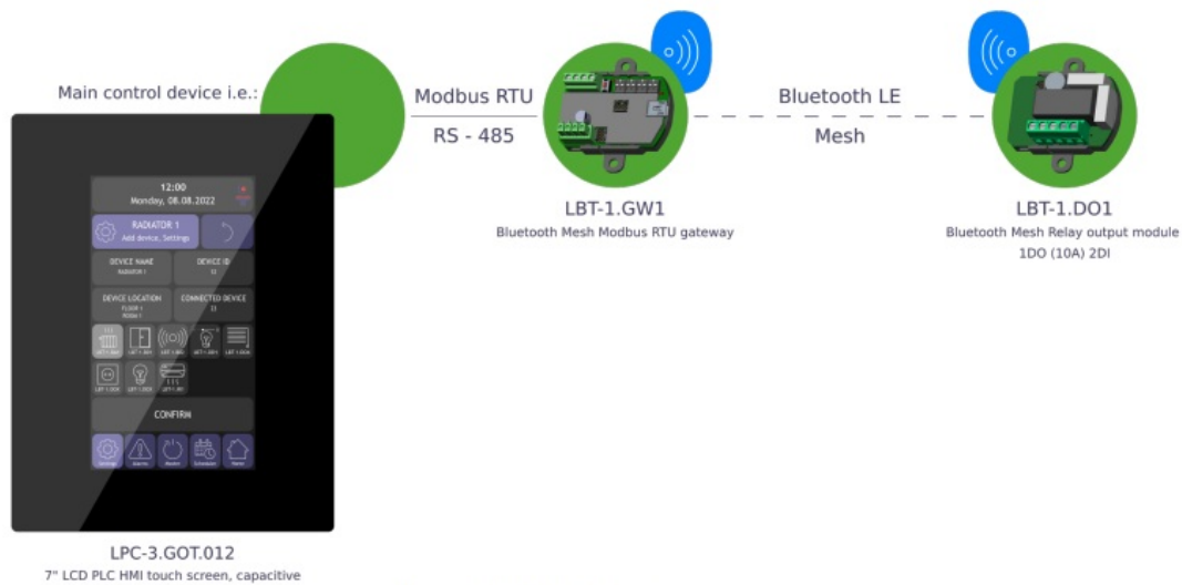
Figure 2: LBT-1.DO1 device connection
