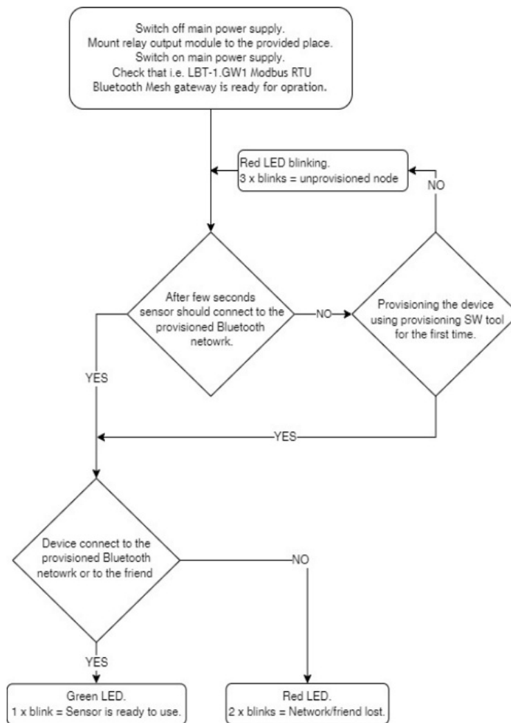
Figure 8: Installation flowchart
