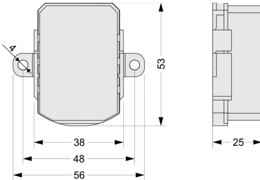
Figure 6: Housing dimensions
