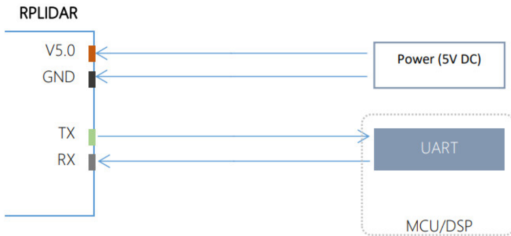
Figure 3-3 RPLIDAR S3 Pins Reference Design
