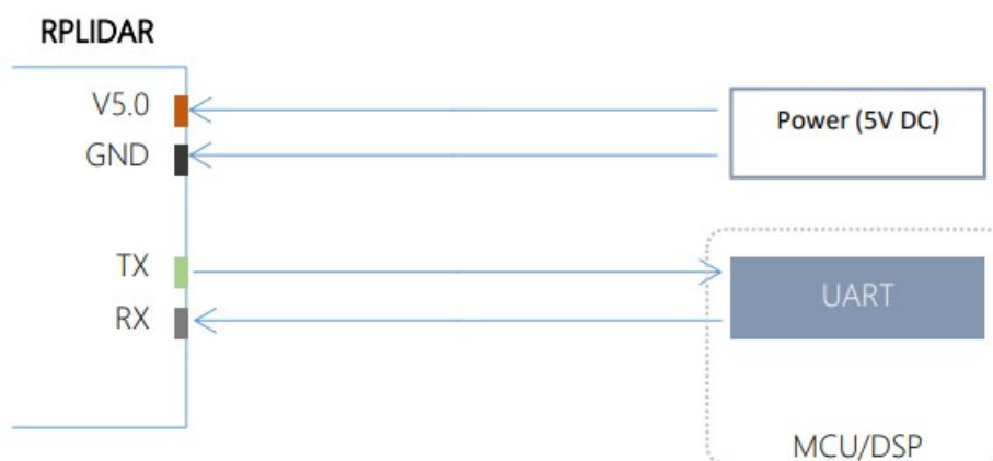
Figure 3-3 RPLIDAR C1 Pins Reference Design
