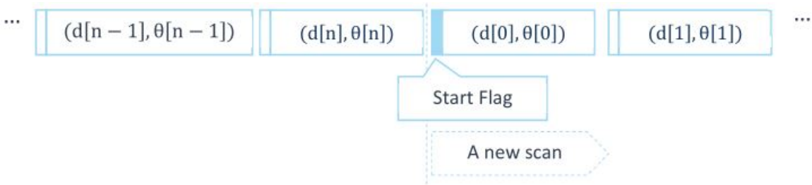
Figure 1-5 The RPLIDAR Sample Point Data Frames
