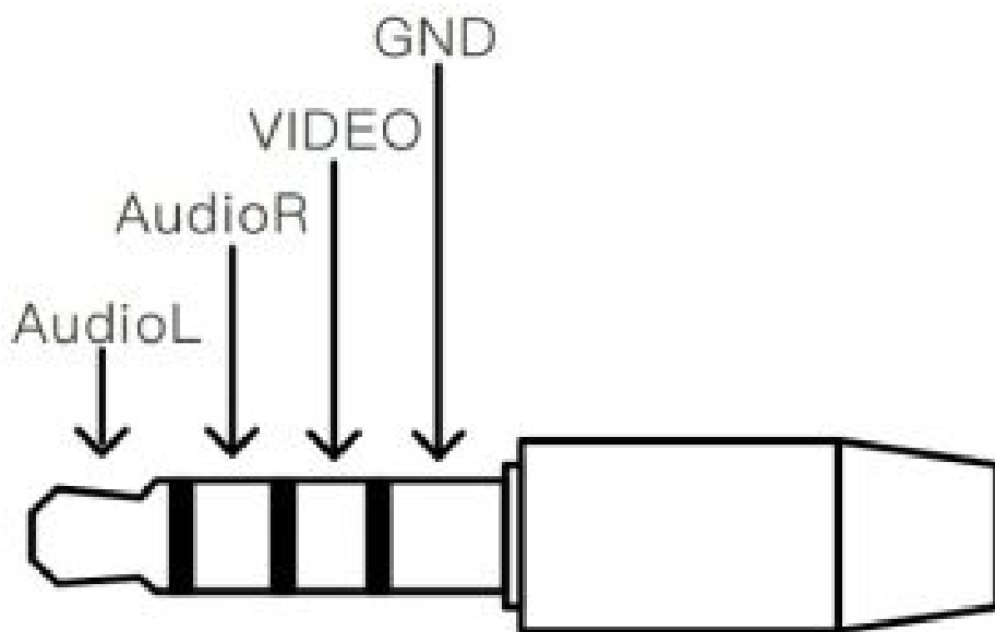
Headtracker Jack Pin-out
