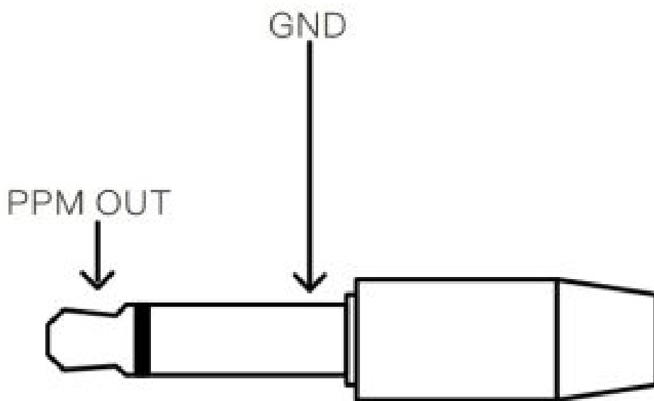
Headtracker Jack Pin-out
