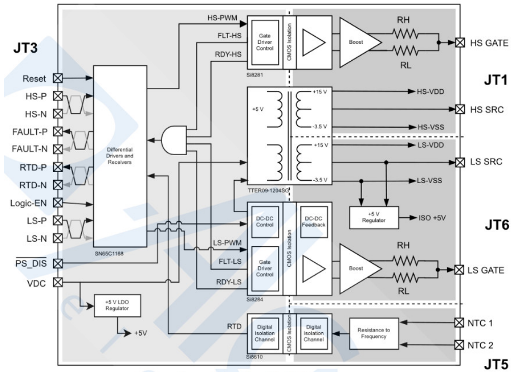
Figure 2. Function Block Diagram
