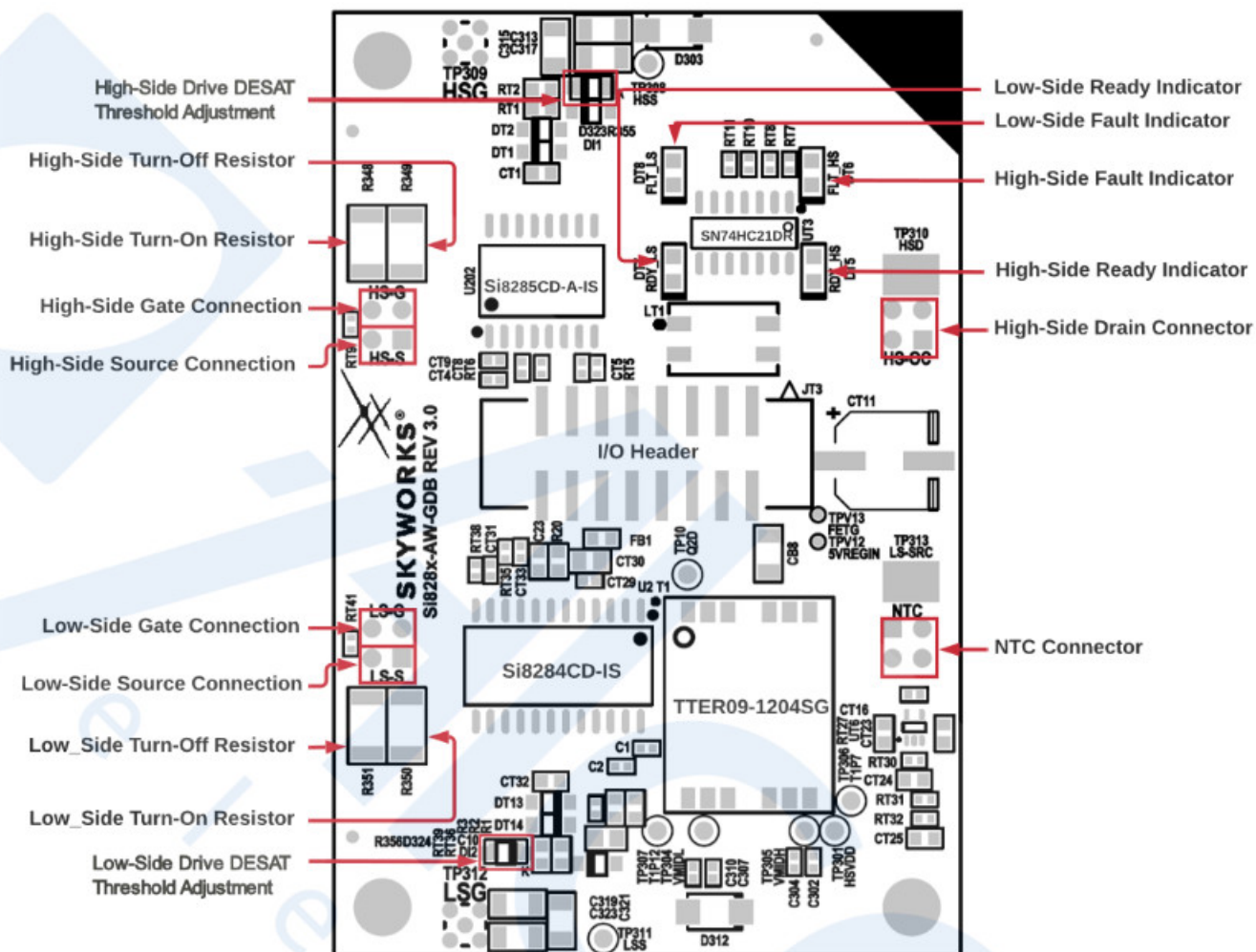
Figure 3. Si828x Gate Driver Board Top-Side Silkscreen
