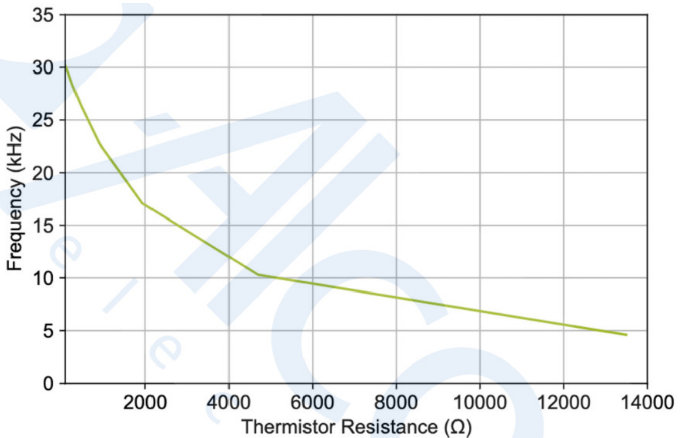
Figure 4. Thermistor Resistance vs Output Frequency
