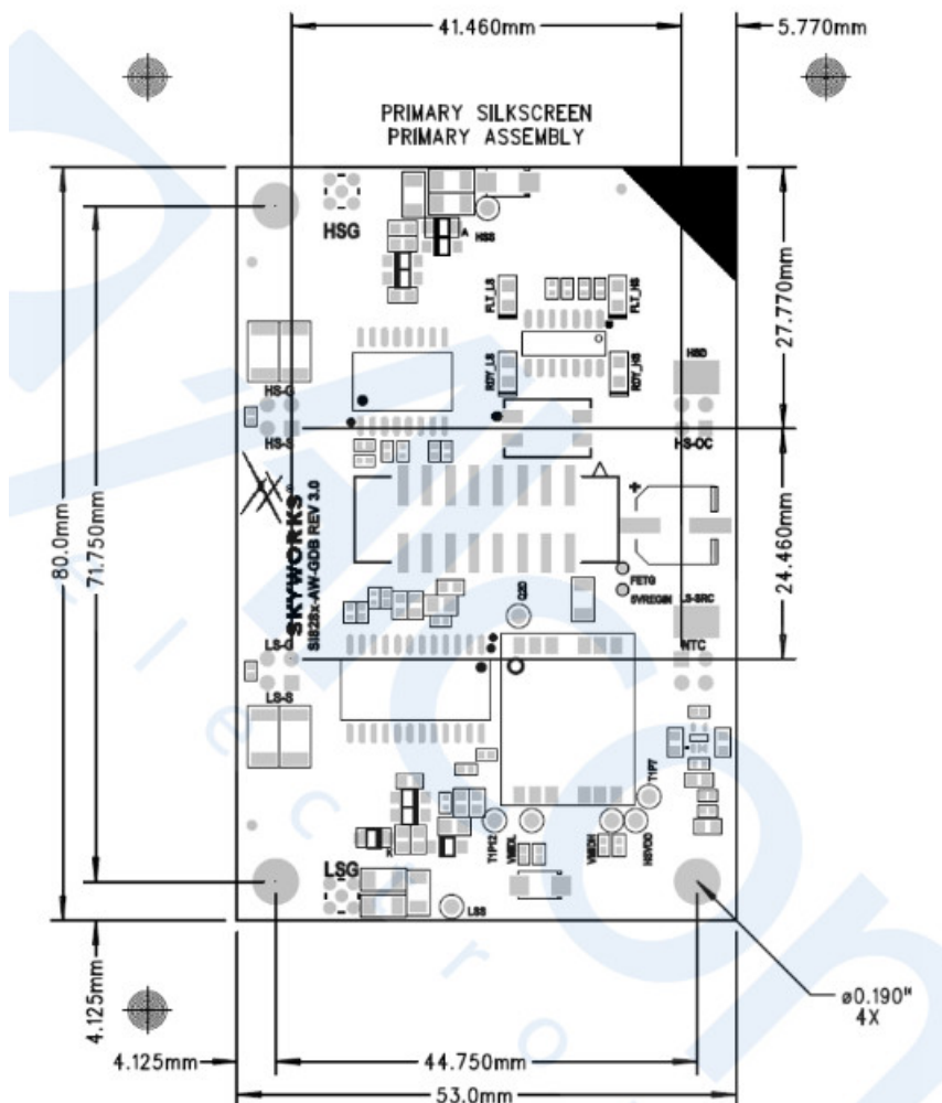
Figure 7. Si828x Gate Driver Board (GDB) Dimensions
