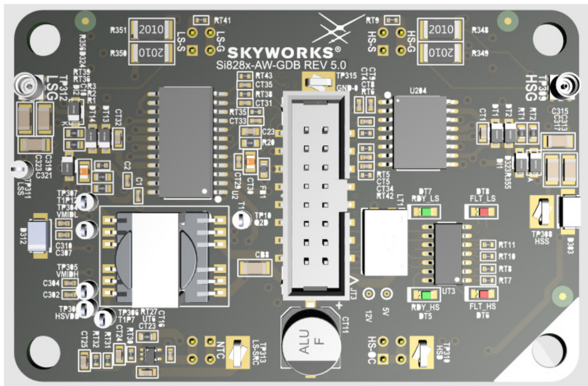
Figure 1. Si828x Gate Driver Board (GDB)
