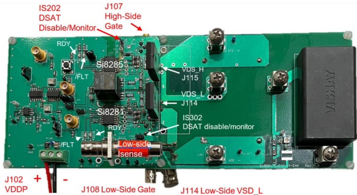
Figure 3.1. Si828x-HB- EVB Scope Probe and DESAT Connections
