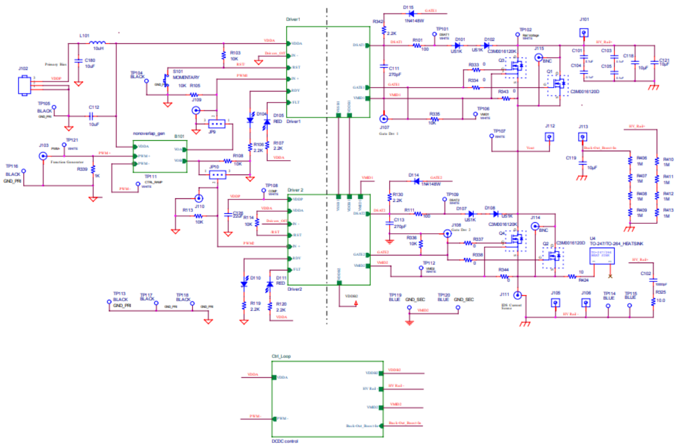
Figure 1.1. Si828x-HB- EVB Half-Bridge Circuit
