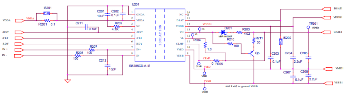
Figure 1.3. High-Side Si8285 Gate Driver (Driver 1)
