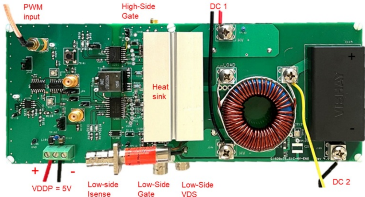
Figure 4.3. Si828x-HB-EVB Buck/Boost DC-DC Operation
