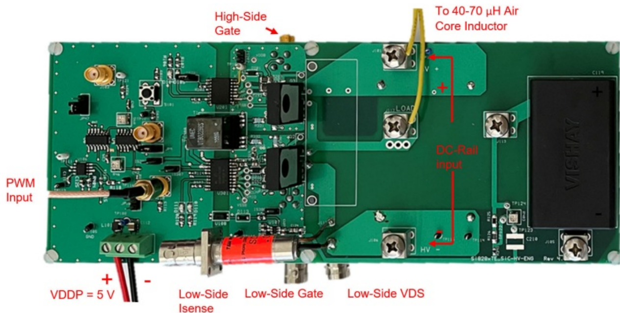
Figure 4.1. Si828x-HB- EVB Connections for Double Pulse Test
