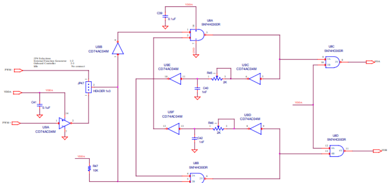
Figure 1.4. Non-Overlap Dead Time Generator Circuit
