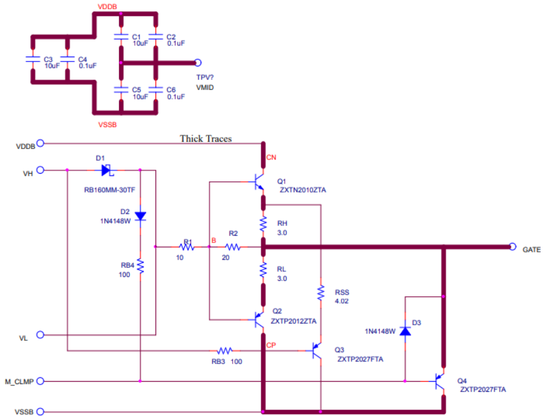
Figure 5.1. Current Booster Circuit
