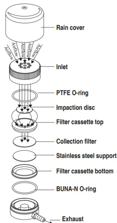
Exploded view of IMPACT Sampler
