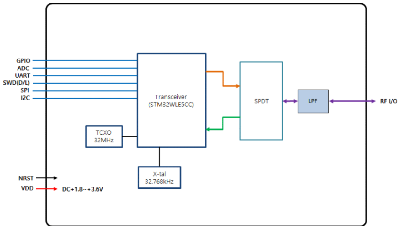
Figure 1-1 LSM110A block diagram and System Interface
