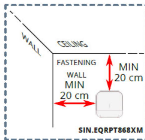
Figure 8 - Wall fixing
