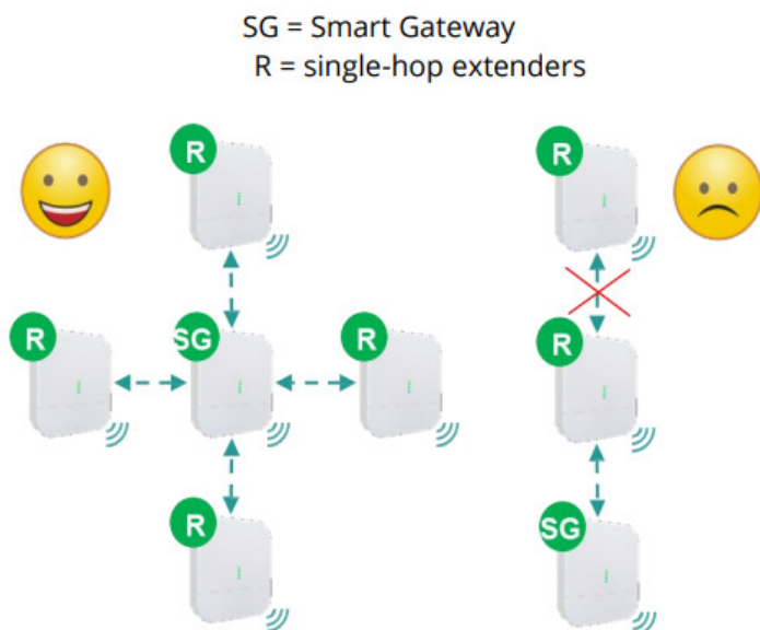
Figure 10 – Connection with extender SIN.EQRPT868X
