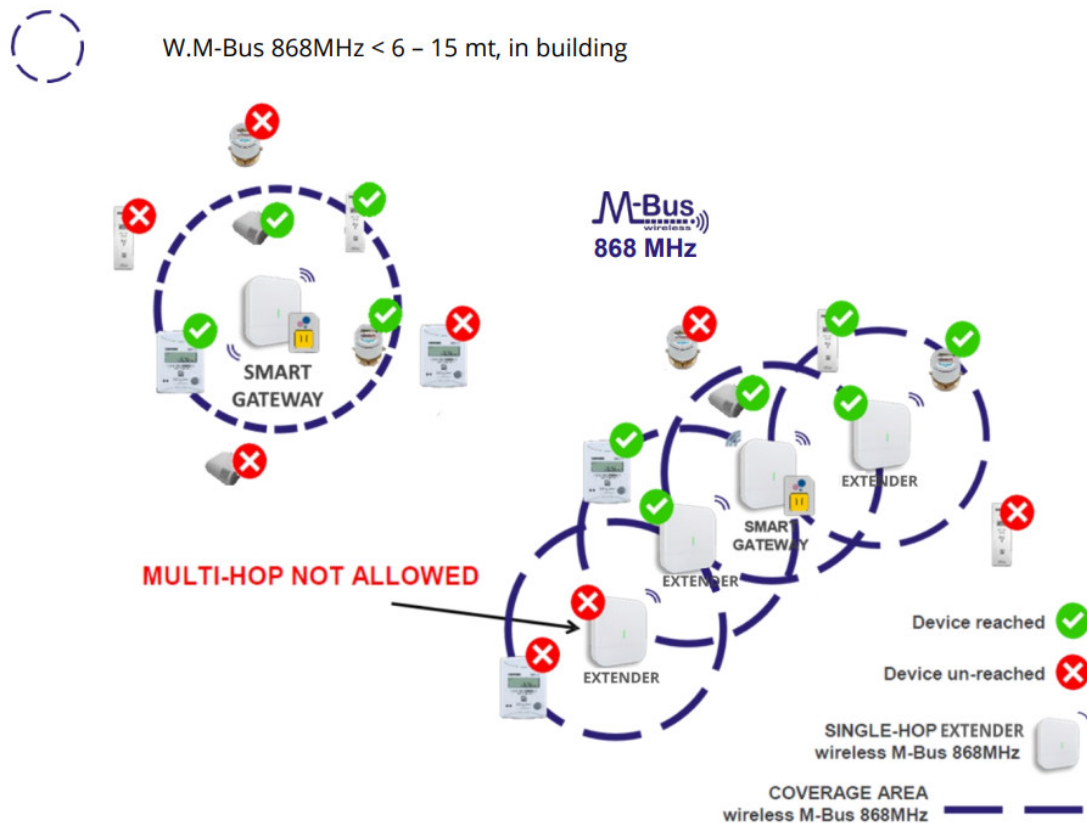
Figure 4 – SIN.EQRPT868XM installation example
