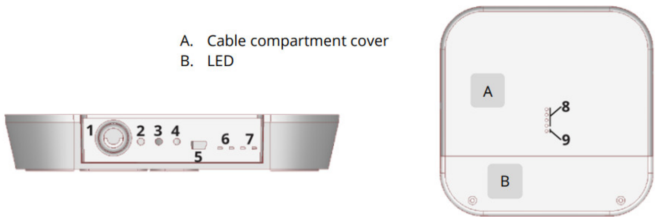
Figure 4 – Connections/push buttons/leds
