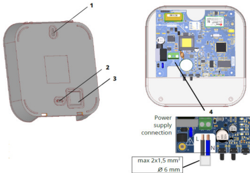
Figure 7 - Cable routing
