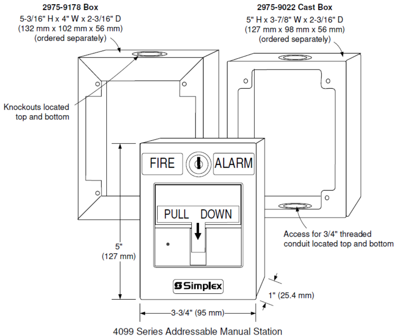
Surface Mount Side View with Internal Detail
