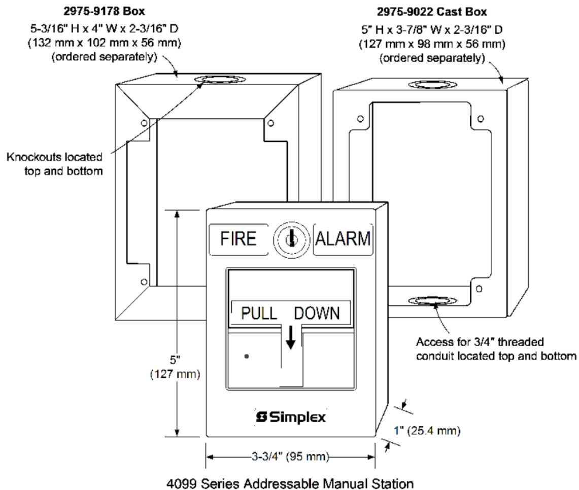
Figure 2: 4099 Series Addressable Manual Station
