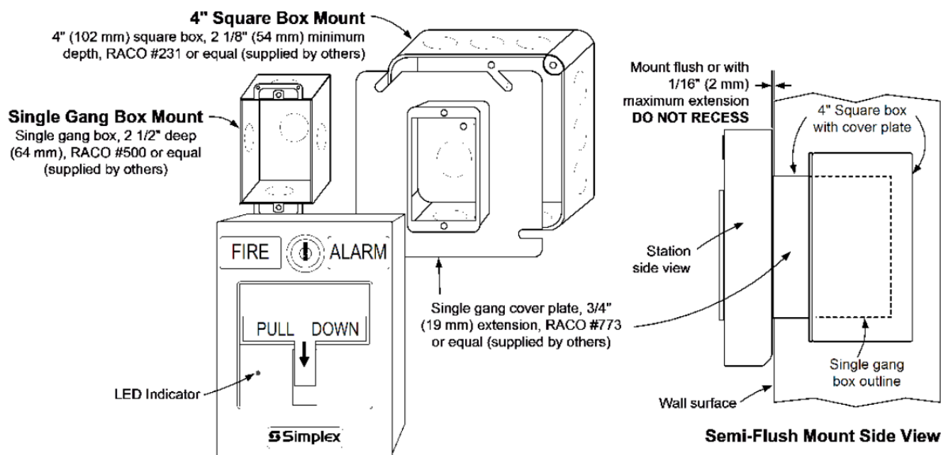
Figure 1: Addressable Manual Station Semi-Flush Mounting
