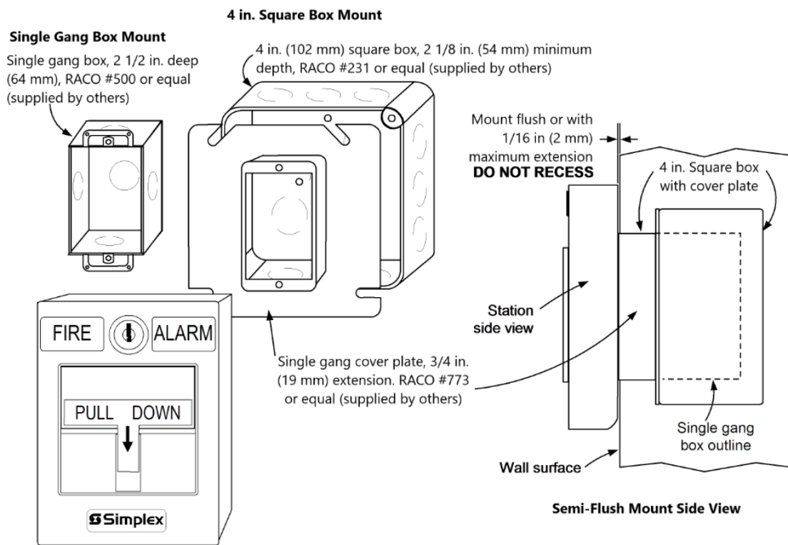
Figure 8: Semi-flush mounting reference
