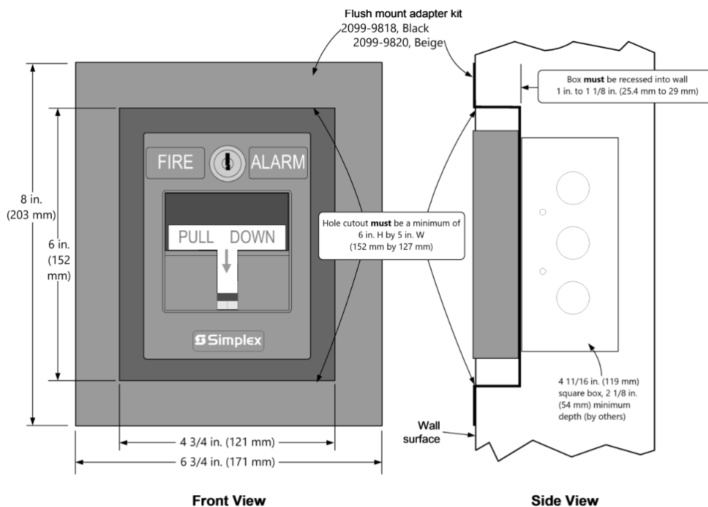
Figure 9: Flush mount reference
