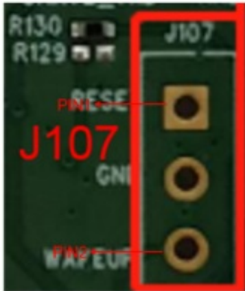
Feature 18: The pin definition of J107 on EVB
