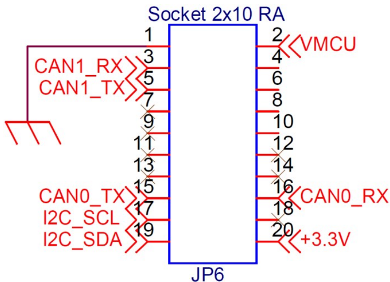
Figure 2.5. EFM32 Giant Gecko 11 STK3701A 20-pin Expansion Header
