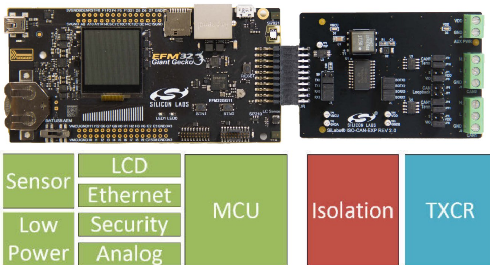
Figure 2.1. MCU + Isolated CAN EXP Block Diagram
