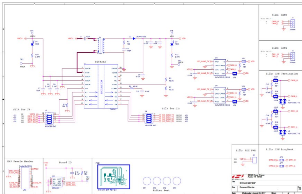
Figure 2.3. Isolated USB EXP Schematic
