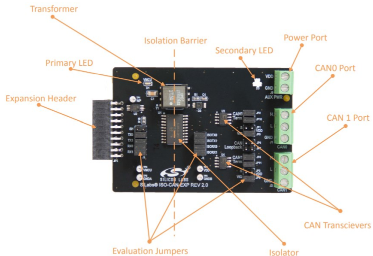
Figure 1.1. Annotated Isolated CAN EXP
