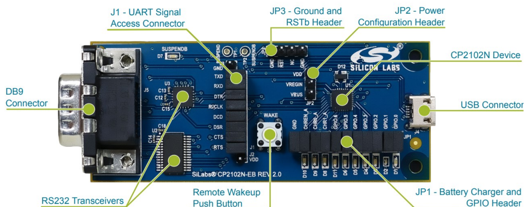
Figure 5.1. CP2102N Evaluation Board
