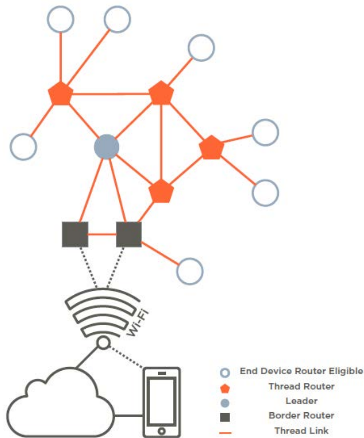
Figure 2.1. Thread Network Architecture
