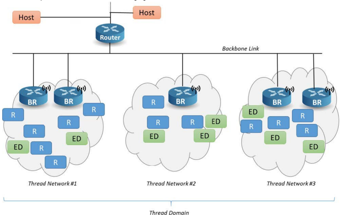
Figure 2.3. Thread Domain Model No Single Point of Failure
