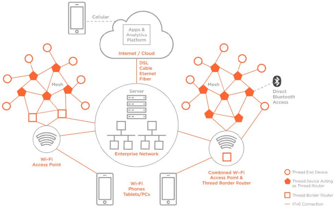
Figure 2.2. Commercial Network Topology
