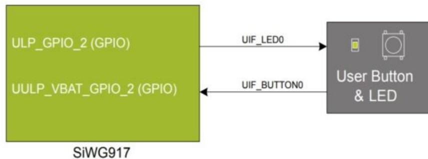
Figure 5.1. Button and LED
