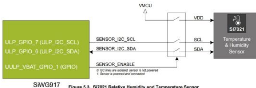
Figure 5.3. Si7021 Relative Humidity and Temperature Sensor
