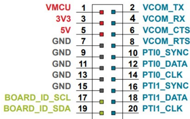
Figure 3.5. Simplicity Connector
