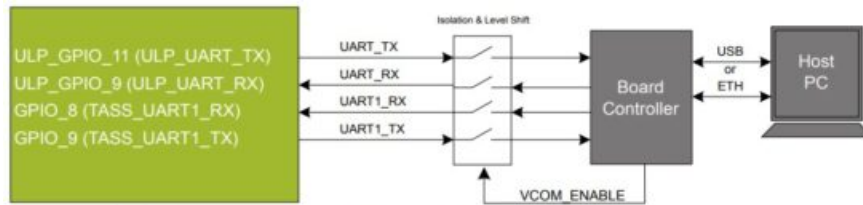
Figure 5.5. Virtual COM Port Interface
