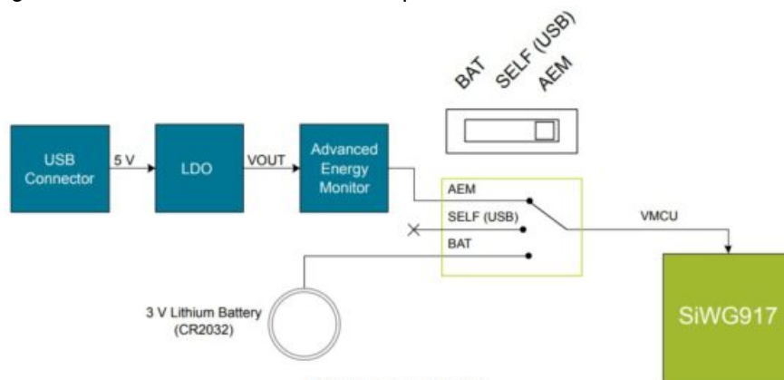
Figure 4.1. Power Switch
