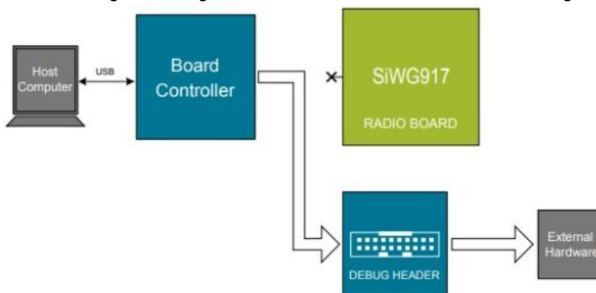
Figure 8.2. Debug OUT
