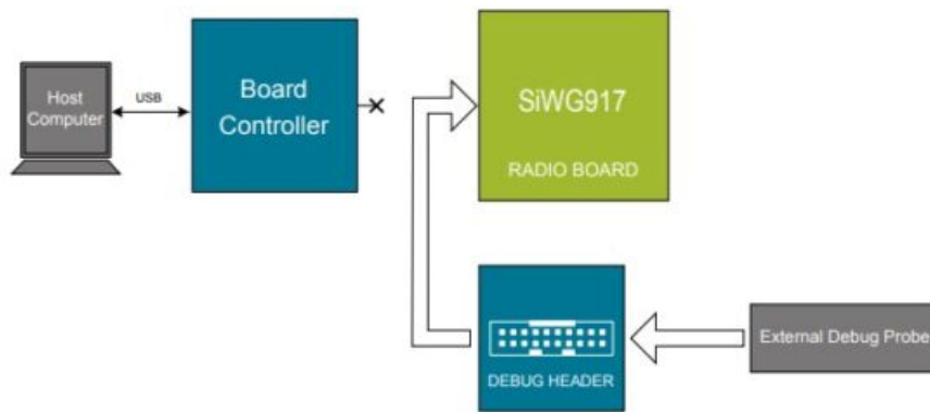
Figure 8.3. Debug IN
