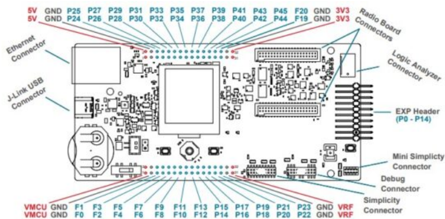
Figure 3.1. Wireless Pro Kit Mainboard (BRD4002A) Connector Layout
