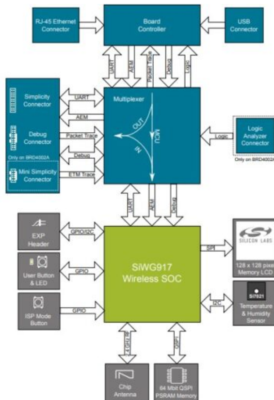
Figure 2.2. Kit Block Diagram
