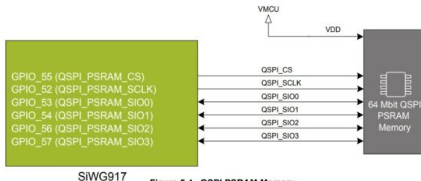
Figure 5.4. QSPI PSRAM Memory
