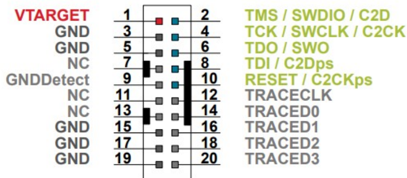
Figure 3.4. Debug Connector
