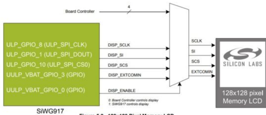
Figure 5.2. 128x128 Pixel Memory LCD
