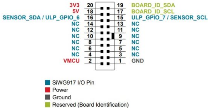
Figure 3.3. EXP Header
