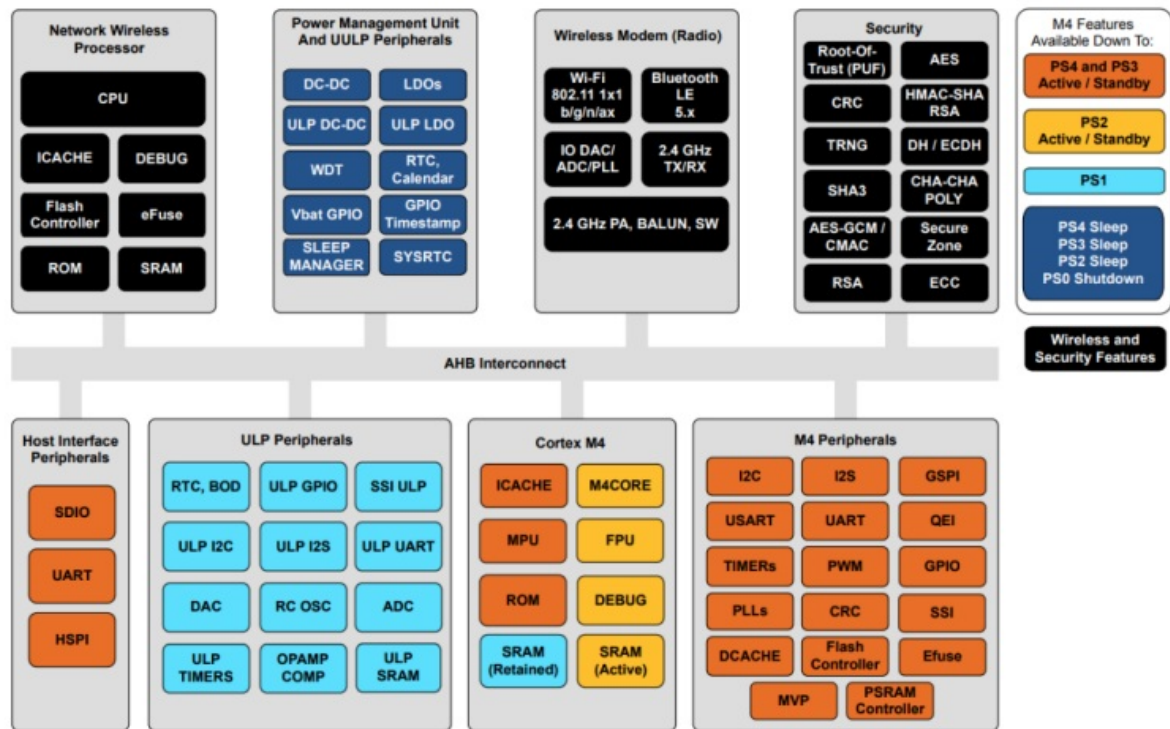
Figure: Low-power Wi-Fi design concept
