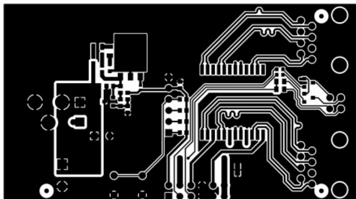
Figure 4.6. Top Layer
