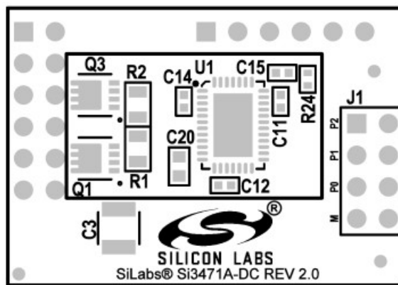
Figure 4.1. Top Silkscreen
