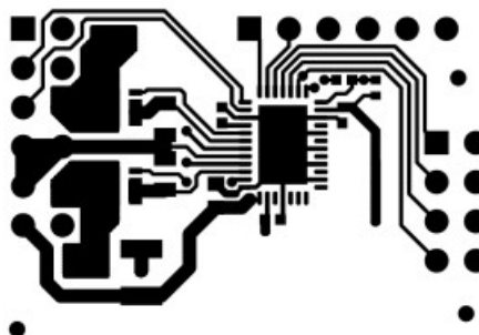
Figure 4.3. Top Layer
