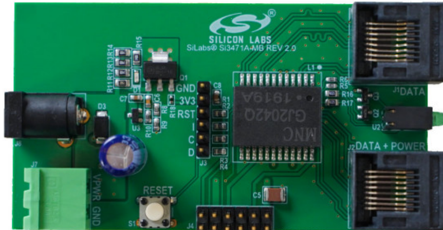
Figure 1.4. Si3471 EVB Baseboard
