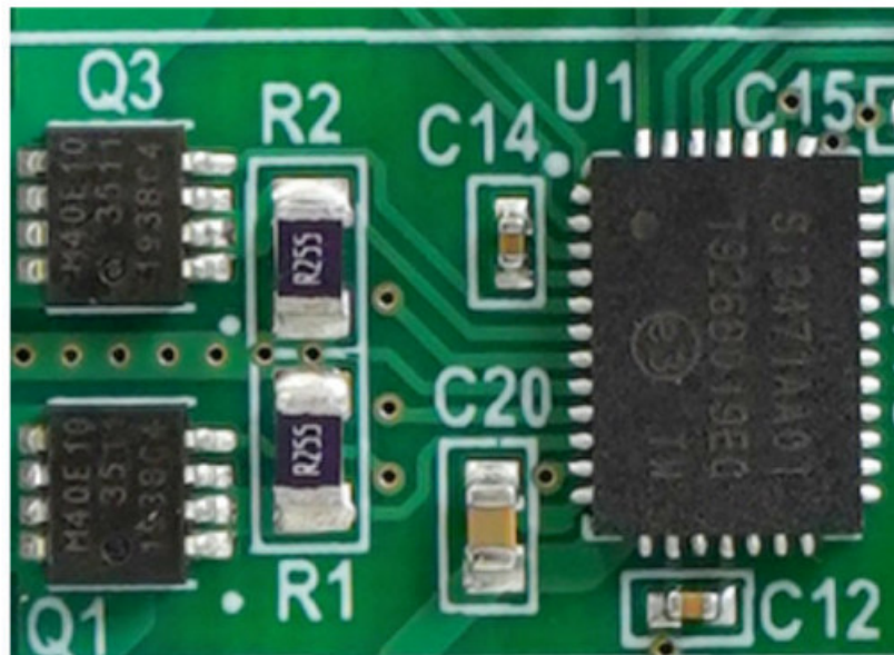
Figure 1.3. Si3471 and External FETs
