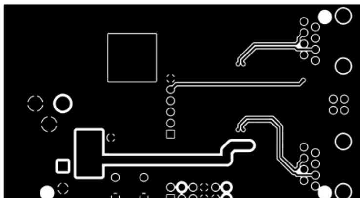
Figure 4.7. Bottom Layer
