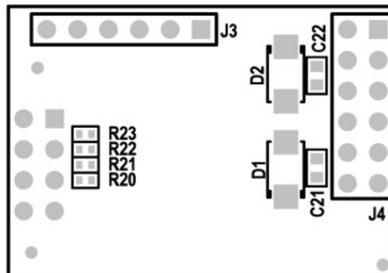
Figure 4.2. Bottom Silkscreen
