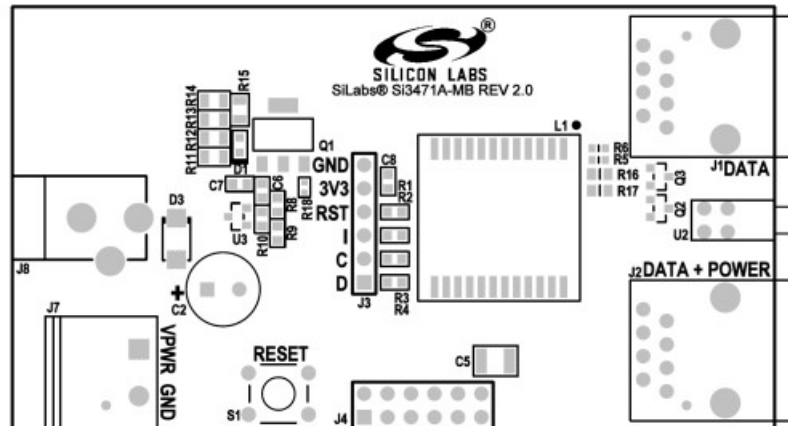
Figure 4.5. Top Silkscreen
