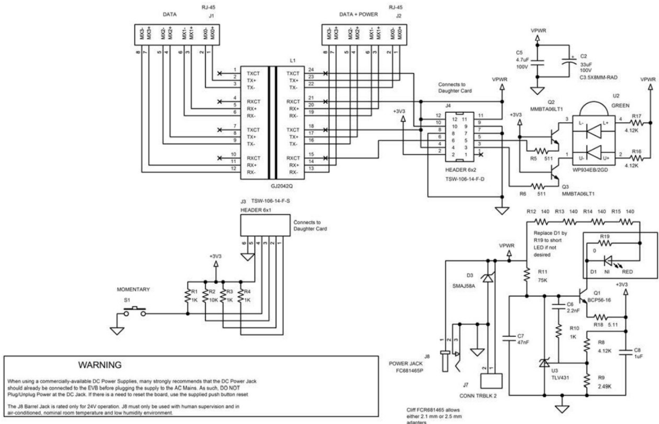
Figure 2.2. Baseboard Schematic
