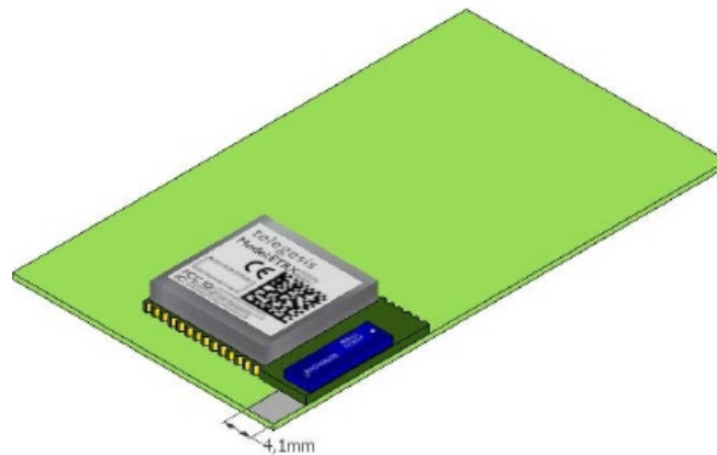
Figure 12. Adding a no copper / no component area
