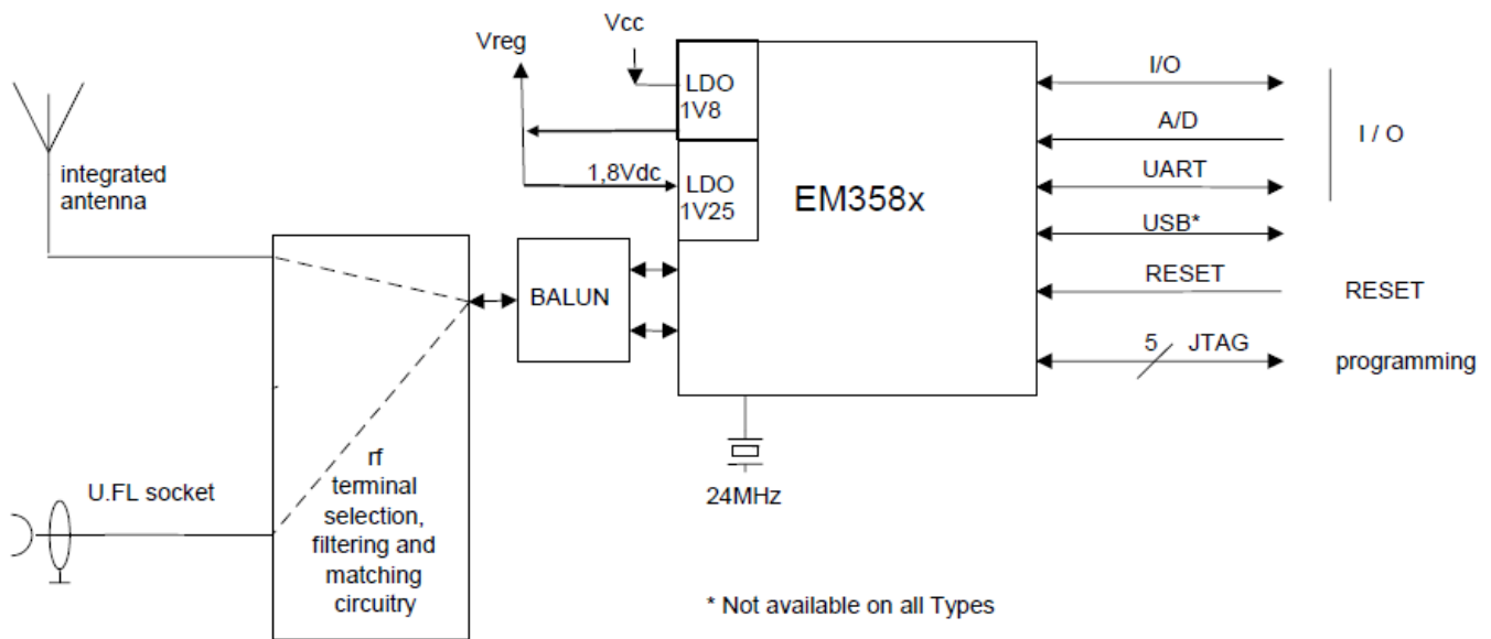
Figure 2: Hardware Diagram
