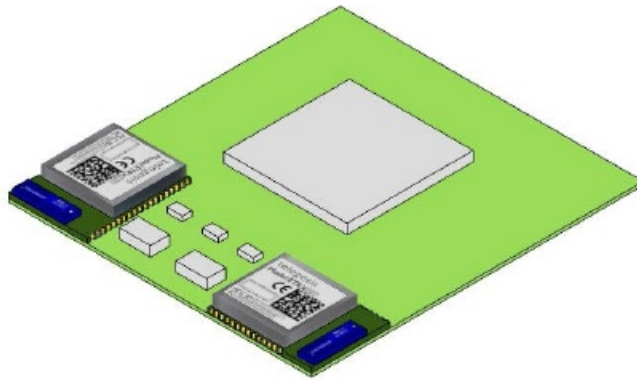
Figure 10. Typical placement
