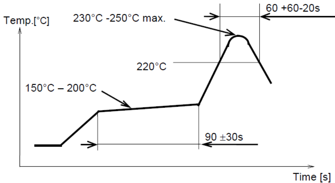
Figure 6. Recommended Reflow Profile
