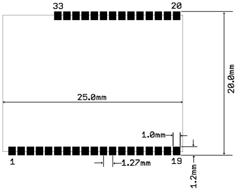
Figure 8: Recommended Footprint
