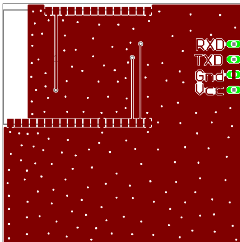
Figure 13. Reference Board
