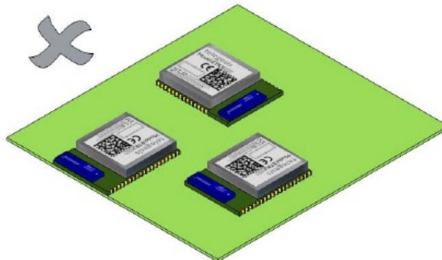
Figure 11. How to not place the Module
