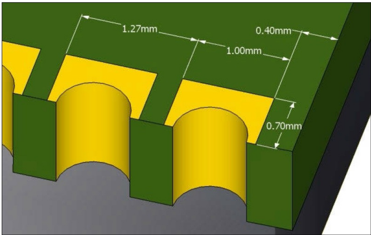
Figure 9. Typical pad dimensions
