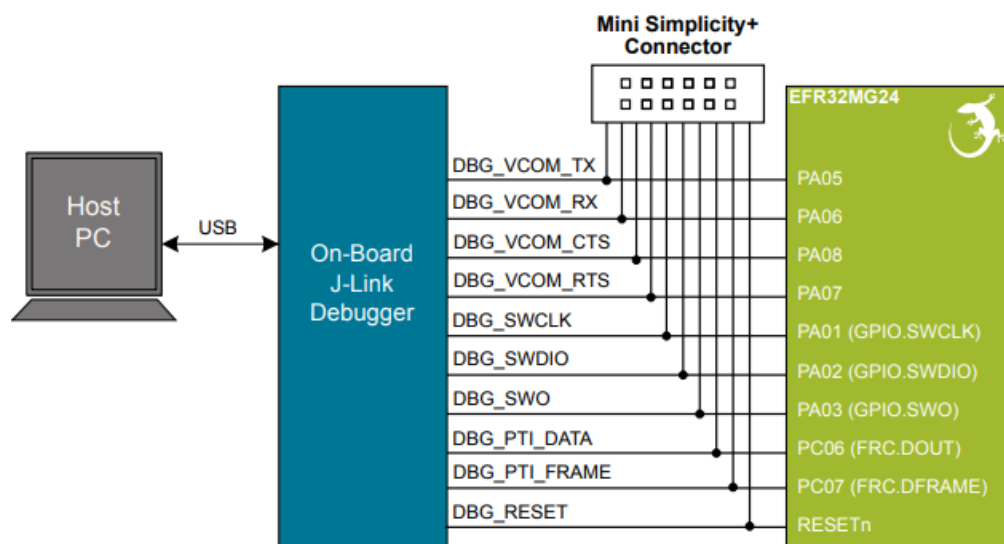
Figure 3.8. On-Board Debugger Connections
