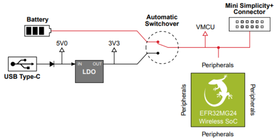
Figure 3.2. EFR32xG24 Channel Sounding Dev Kit Power Architecture
