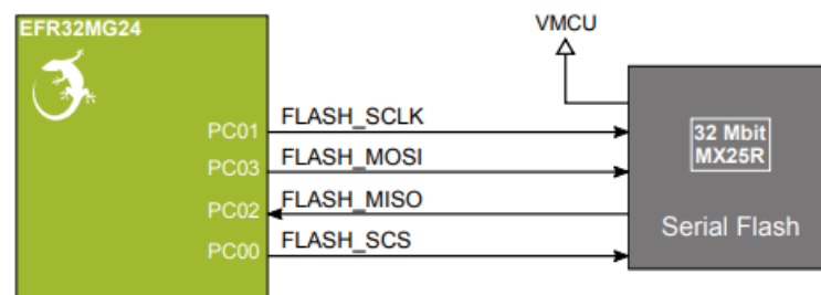
Figure 3.6. Serial Flash
