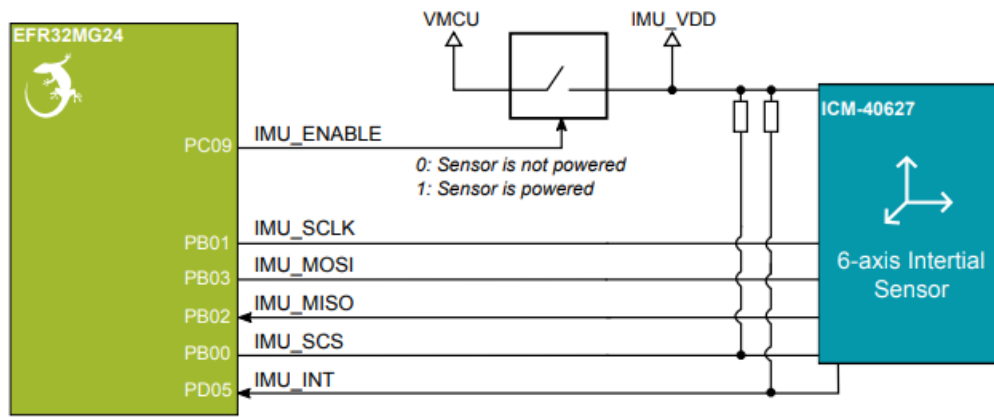
Figure 3.4. ICM-40627 6-Axis Inertial Sensor
