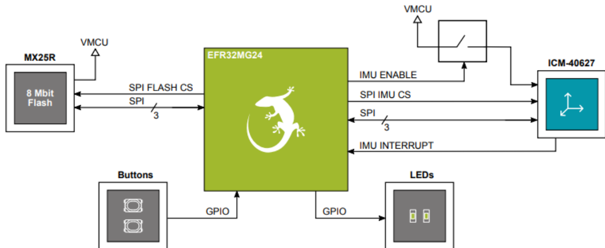
Figure 3.3. Peripherals
