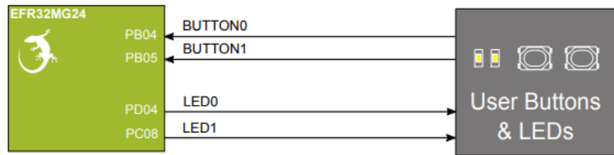
Figure 3.7. Buttons and LEDs
