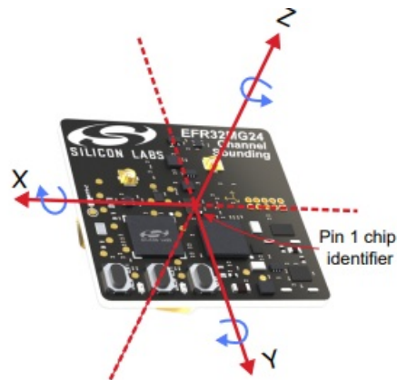
Figure 3.5. EFR32xG24 Channel Sounding Dev Kit Spatial Orientation
