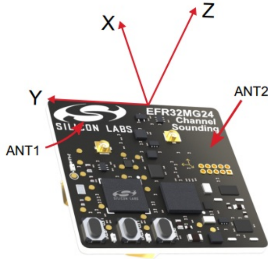
Figure 5.2. DUT Reference Planes and Printed Antenna Locations
