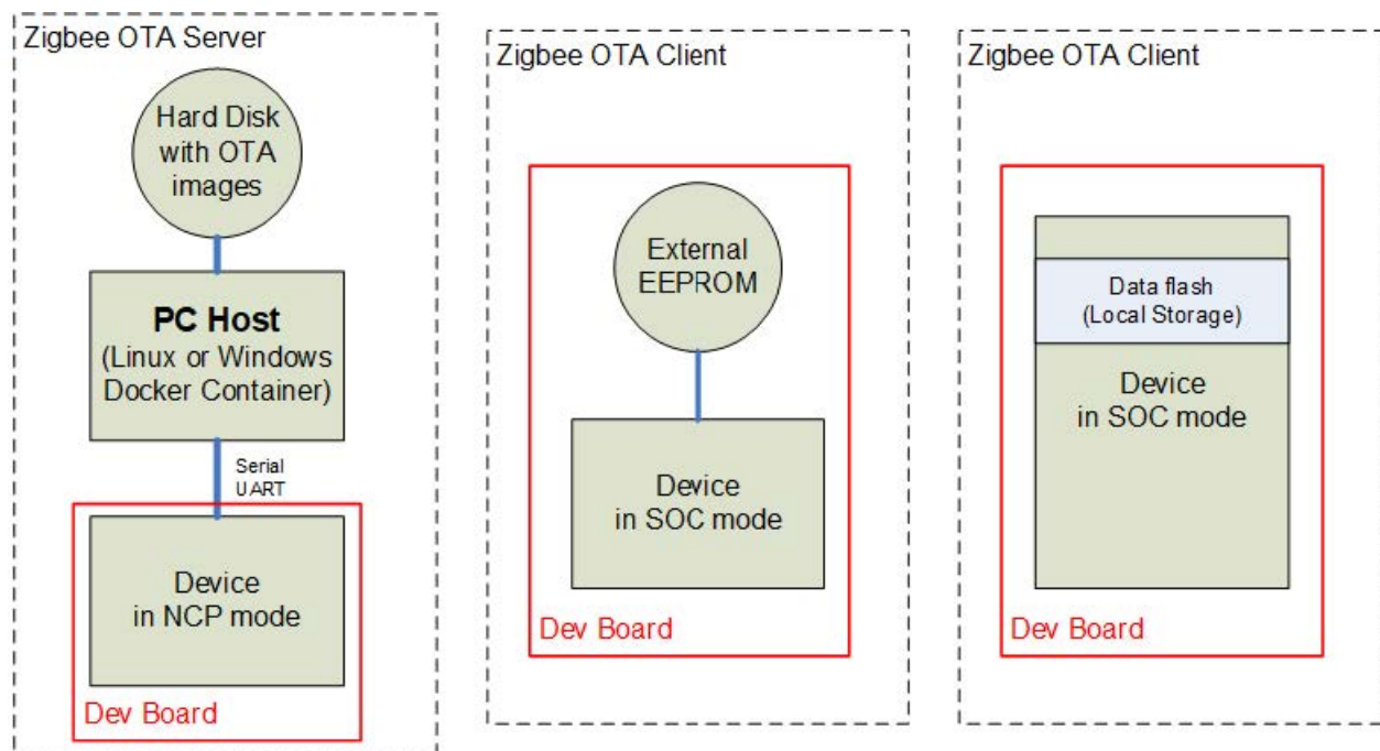
Figure 2.1. Zigbee OTA Application Bootload Hardware Diagram
